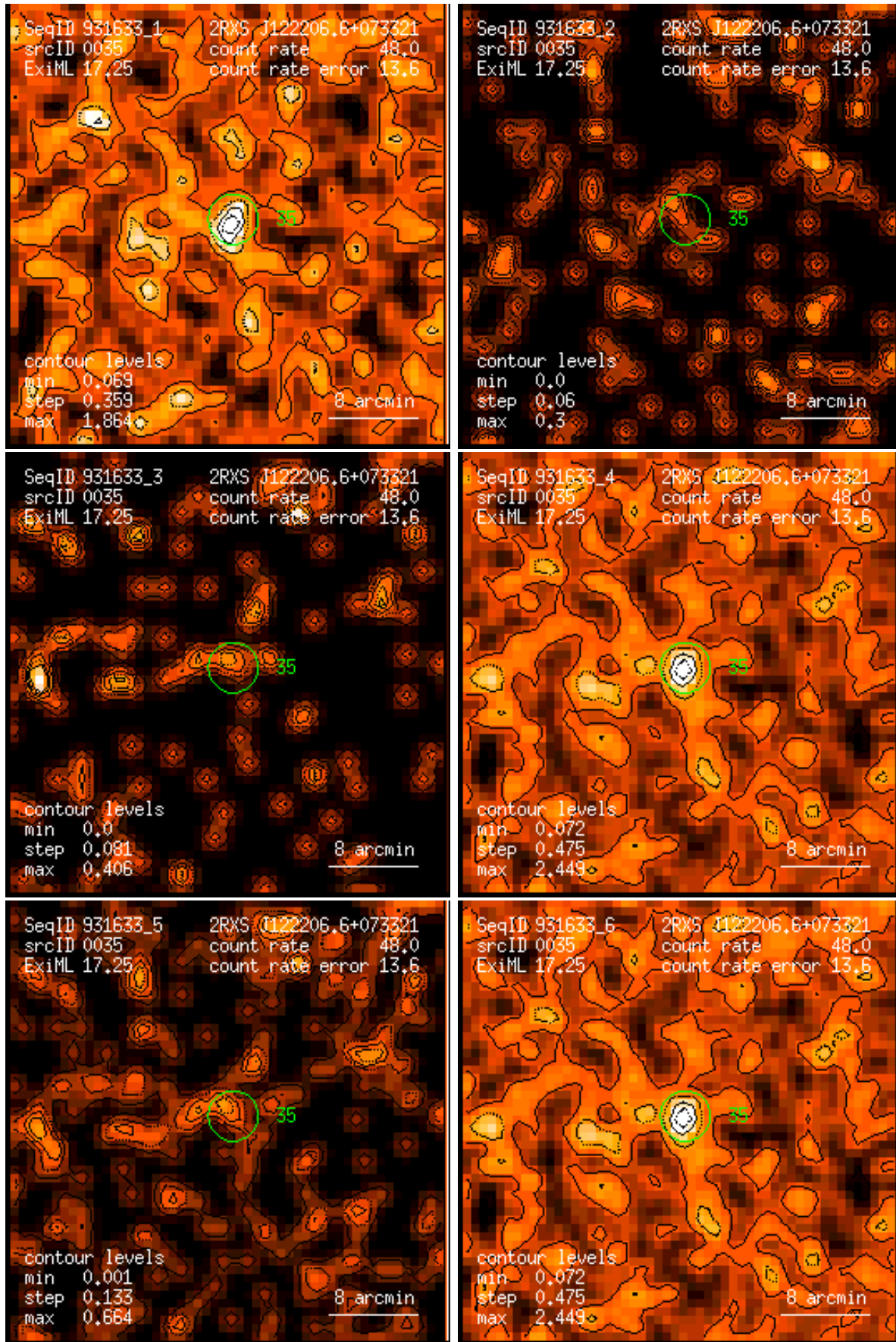
Figure 35: RASS 931633: detection 0035: band rate images, Gaussian filter: (1) PSPC channels 11 – 41, (2) 52 – 90, (3) 91 – 201, (4) 11 – 235, (5) 52 – 201, (6) 11 – 201. Broad band rates in counts/ks. Band rate contour levels in counts/ks/arcmin 2 .
