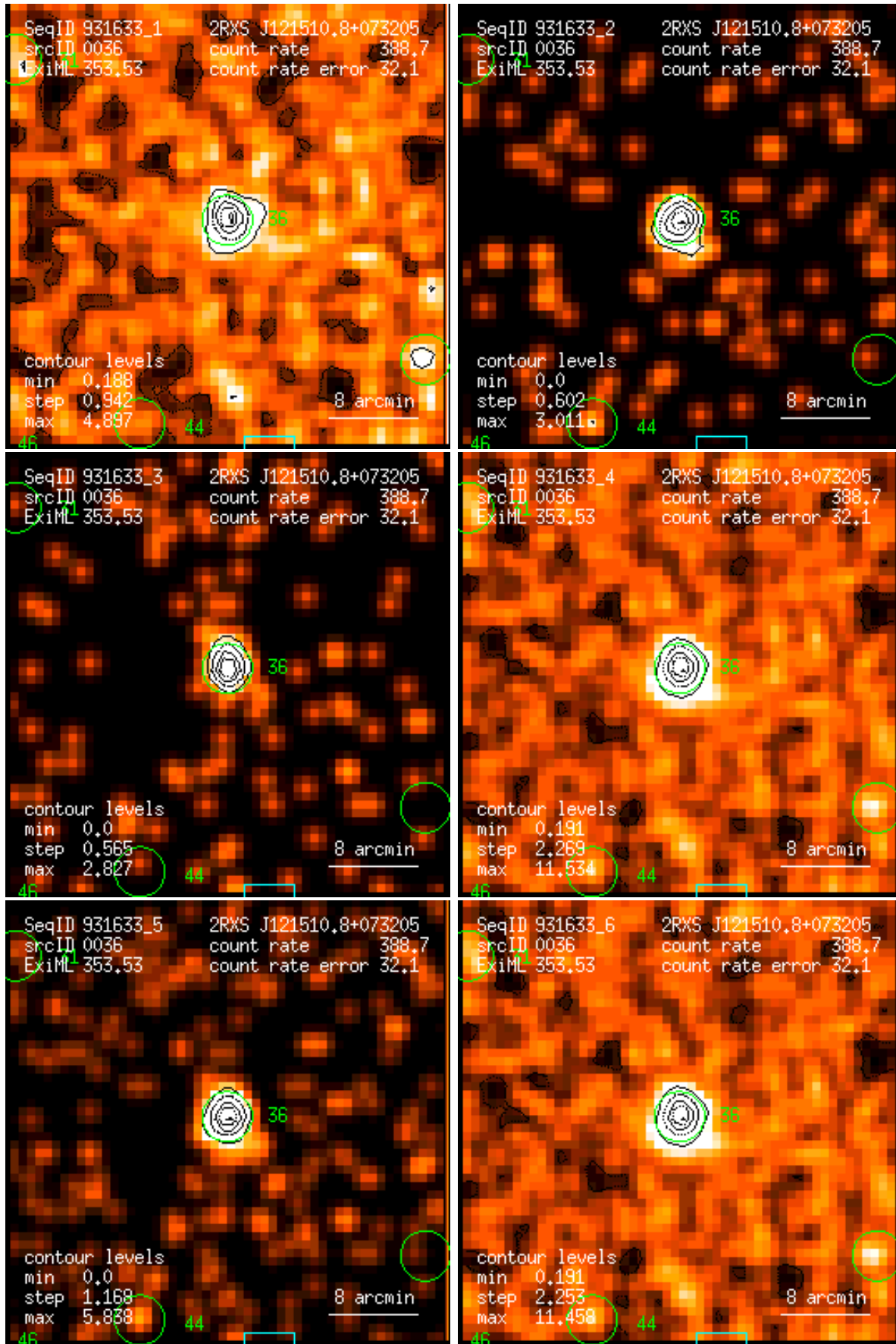
Figure 36: RASS 931633: detection 0036: band rate images, Gaussian filter: (1) PSPC channels 11 – 41, (2) 52 – 90, (3) 91 – 201, (4) 11 – 235, (5) 52 – 201, (6) 11 – 201. Broad band rates in counts/ks. Band rate contour levels in counts/ks/arcmin 2 .
