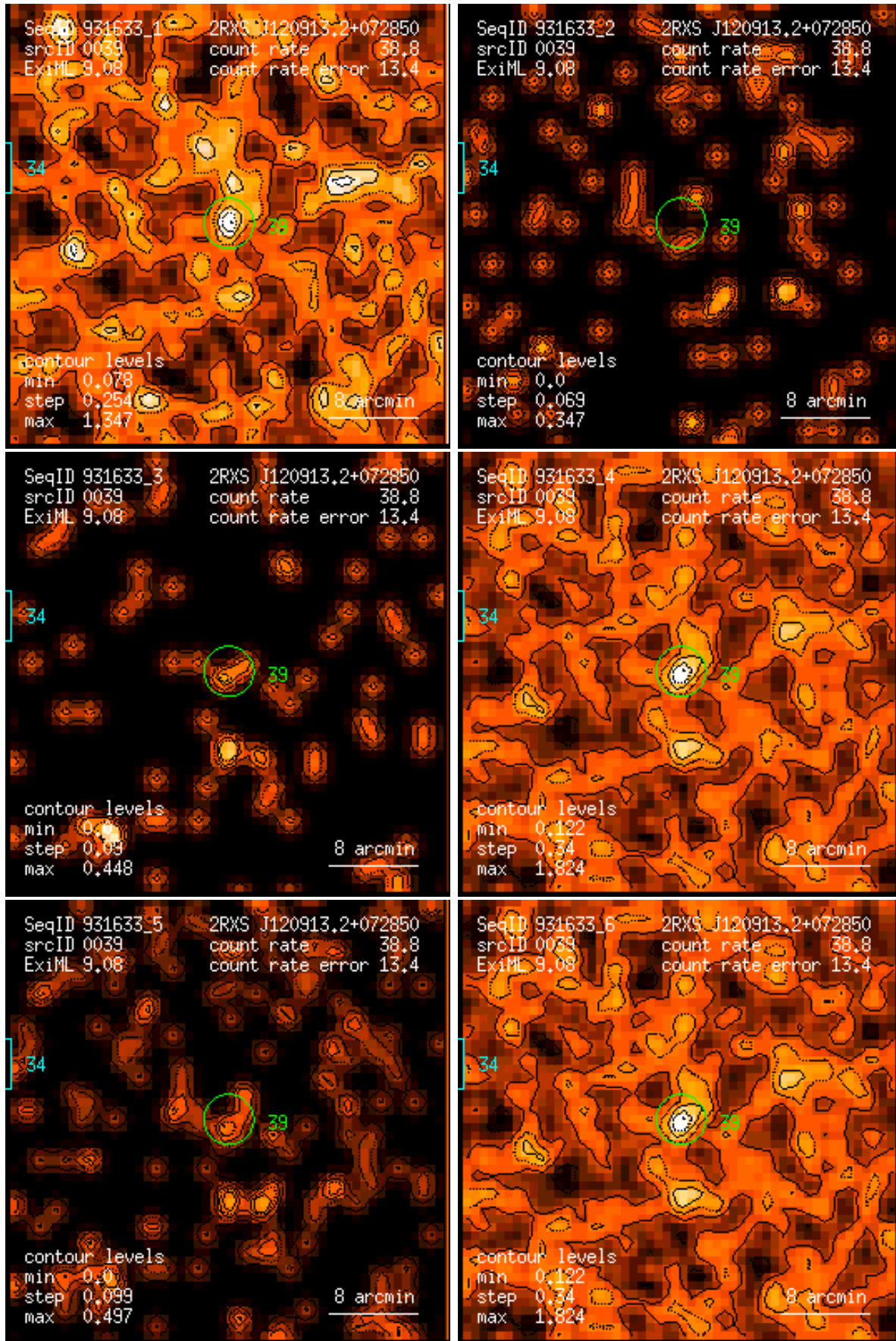
Figure 39: RASS 931633: detection 0039: band rate images, Gaussian filter: (1) PSPC channels 11 – 41, (2) 52 – 90, (3) 91 – 201, (4) 11 – 235, (5) 52 – 201, (6) 11 – 201. Broad band rates in counts/ks. Band rate contour levels in counts/ks/arcmin 2 .
