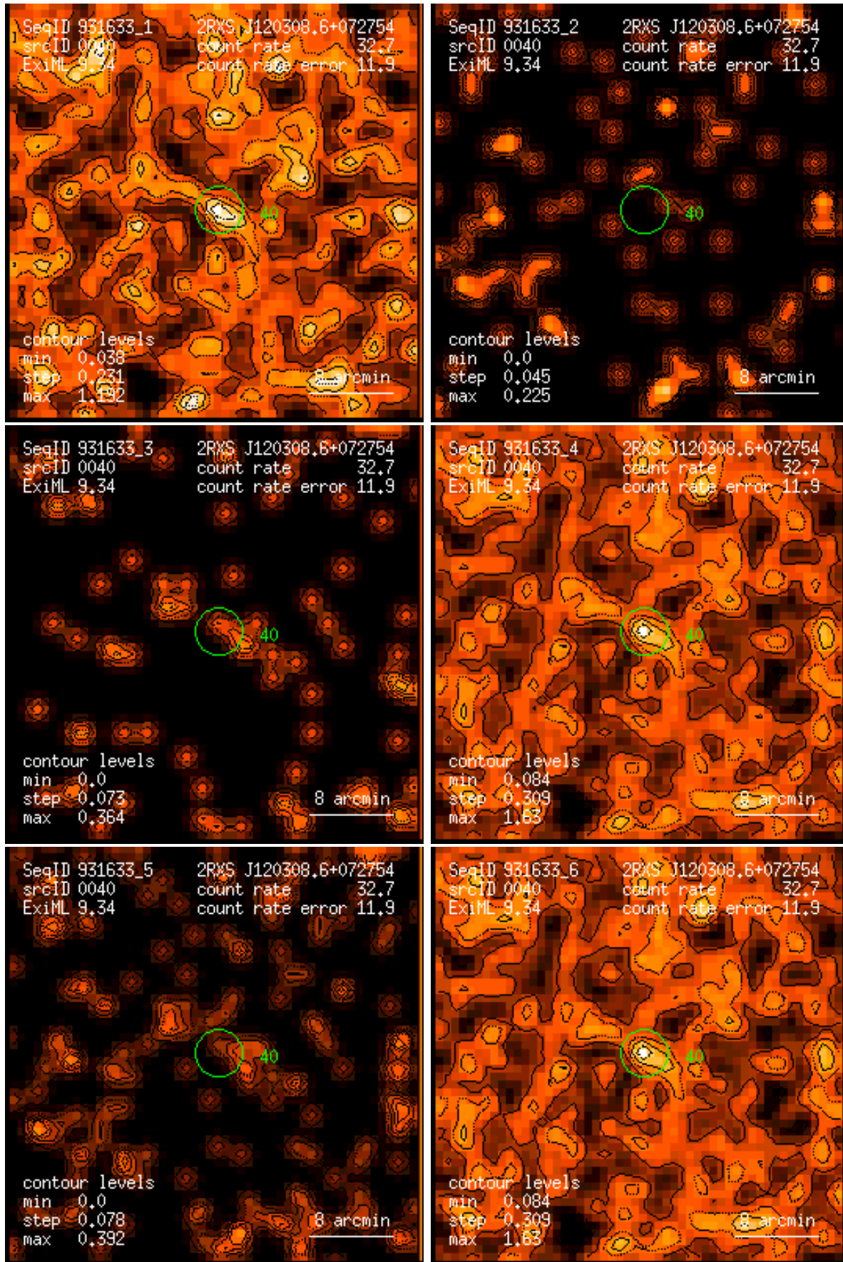
Figure 40: RASS 931633: detection 0040: band rate images, Gaussian filter: (1) PSPC channels 11 – 41, (2) 52 – 90, (3) 91 – 201, (4) 11 – 235, (5) 52 – 201, (6) 11 – 201. Broad band rates in counts/ks. Band rate contour levels in counts/ks/arcmin 2 .
