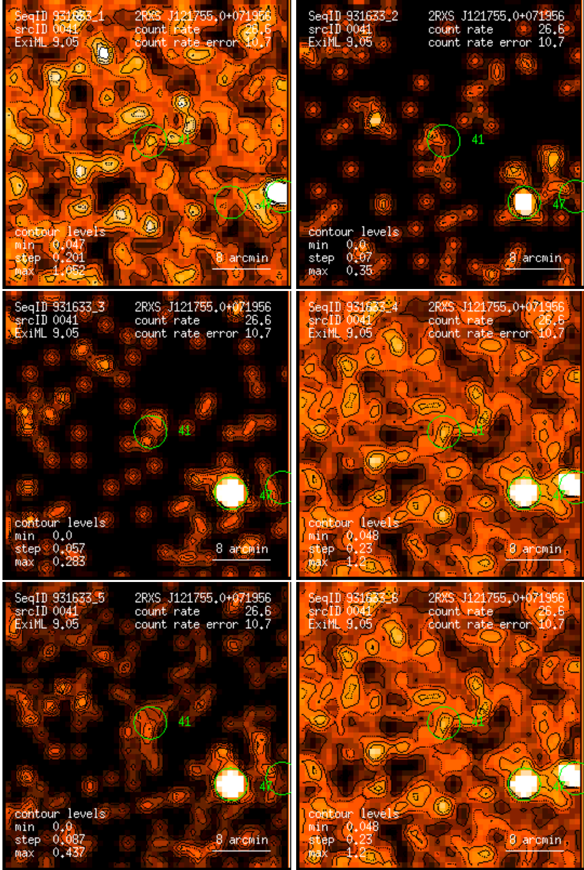
Figure 41: RASS 931633: detection 0041: band rate images, Gaussian filter: (1) PSPC channels 11 – 41, (2) 52 – 90, (3) 91 – 201, (4) 11 – 235, (5) 52 – 201, (6) 11 – 201. Broad band rates in counts/ks. Band rate contour levels in counts/ks/arcmin 2 .
