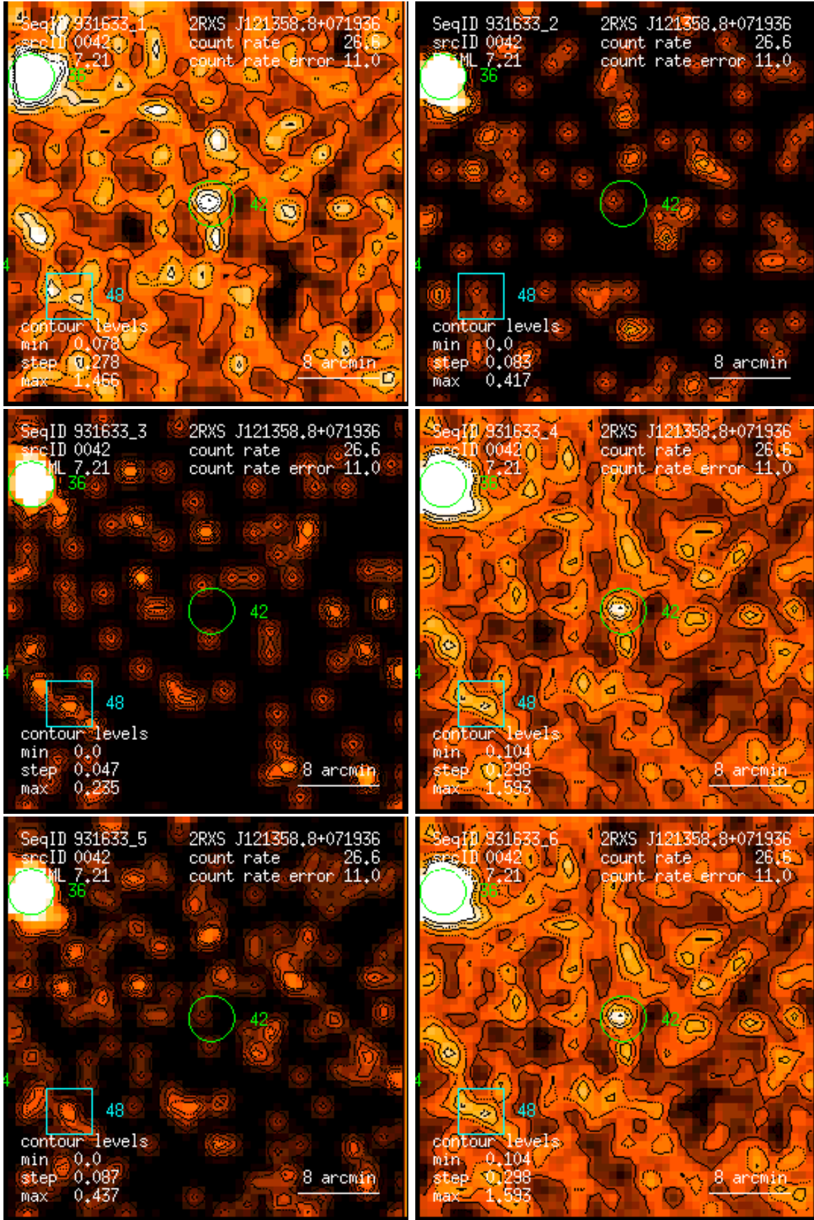
Figure 42: RASS 931633: detection 0042: band rate images, Gaussian filter: (1) PSPC channels 11 – 41, (2) 52 – 90, (3) 91 – 201, (4) 11 – 235, (5) 52 – 201, (6) 11 – 201. Broad band rates in counts/ks. Band rate contour levels in counts/ks/arcmin 2 .
