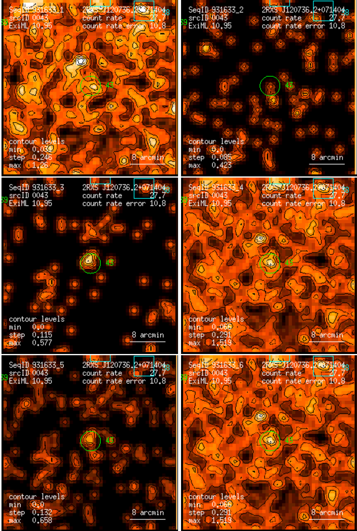
Figure 43: RASS 931633: detection 0043: band rate images, Gaussian filter: (1) PSPC channels 11 – 41, (2) 52 – 90, (3) 91 – 201, (4) 11 – 235, (5) 52 – 201, (6) 11 – 201. Broad band rates in counts/ks. Band rate contour levels in counts/ks/arcmin 2 .
