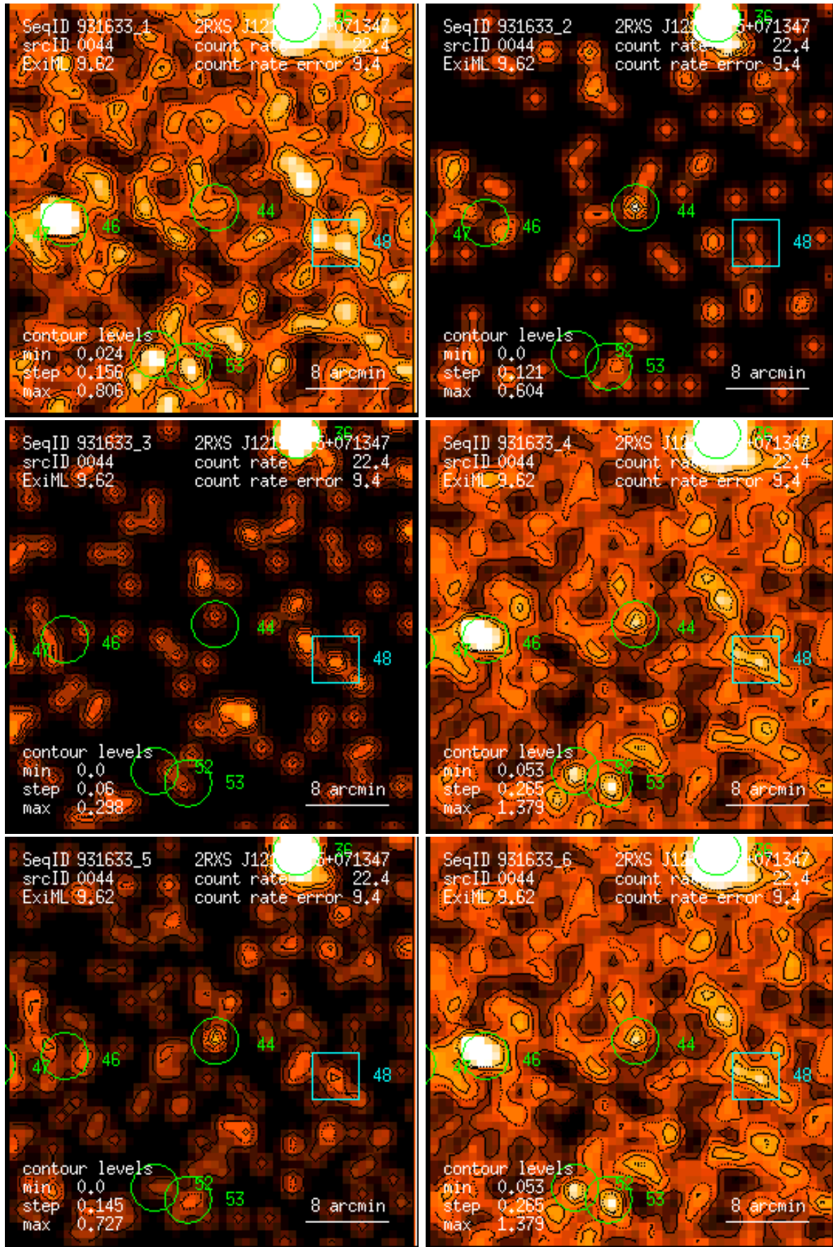
Figure 44: RASS 931633: detection 0044: band rate images, Gaussian filter: (1) PSPC channels 11 – 41, (2) 52 – 90, (3) 91 – 201, (4) 11 – 235, (5) 52 – 201, (6) 11 – 201. Broad band rates in counts/ks. Band rate contour levels in counts/ks/arcmin 2 .
