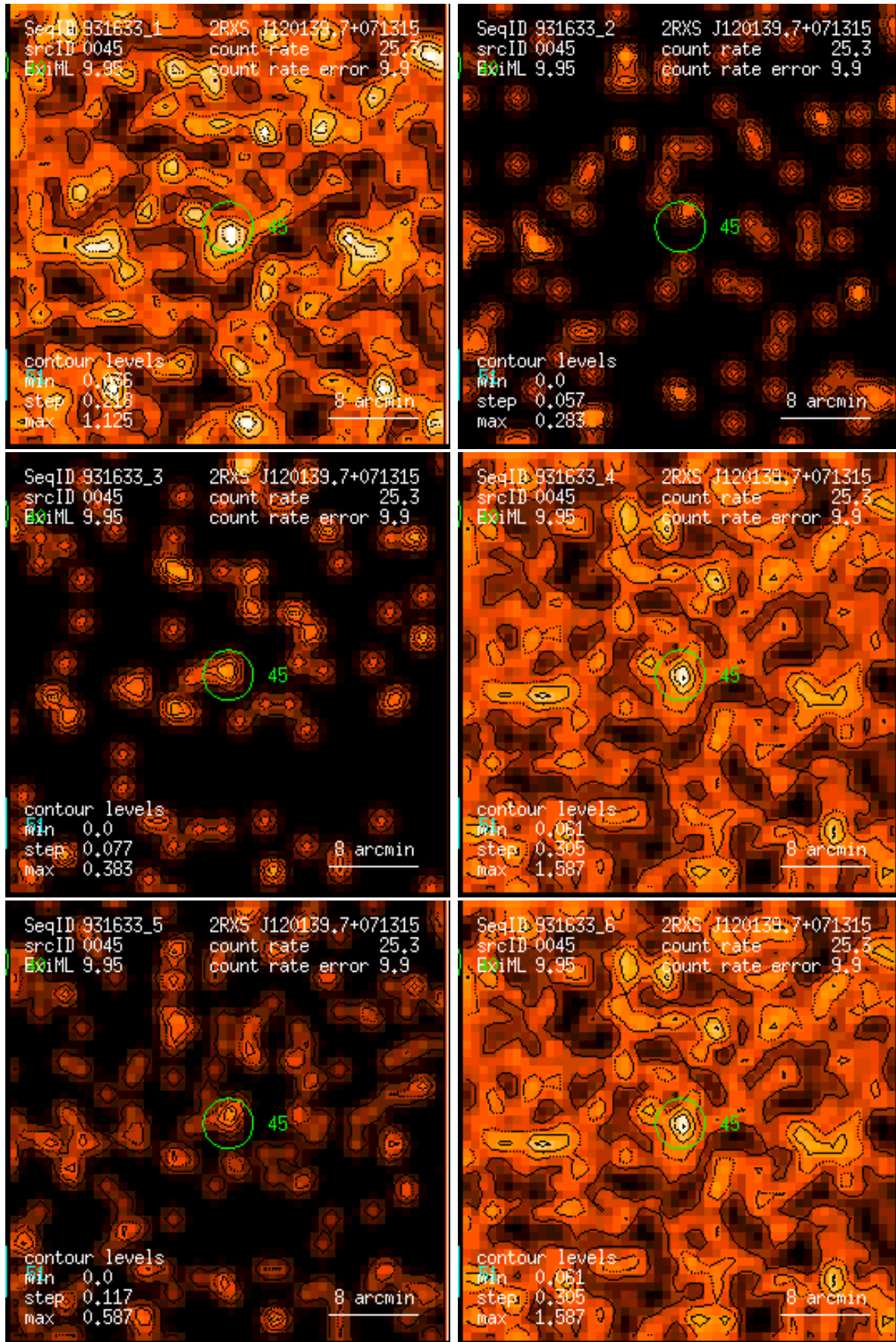
Figure 45: RASS 931633: detection 0045: band rate images, Gaussian filter: (1) PSPC channels 11 – 41, (2) 52 – 90, (3) 91 – 201, (4) 11 – 235, (5) 52 – 201, (6) 11 – 201. Broad band rates in counts/ks. Band rate contour levels in counts/ks/arcmin 2 .
