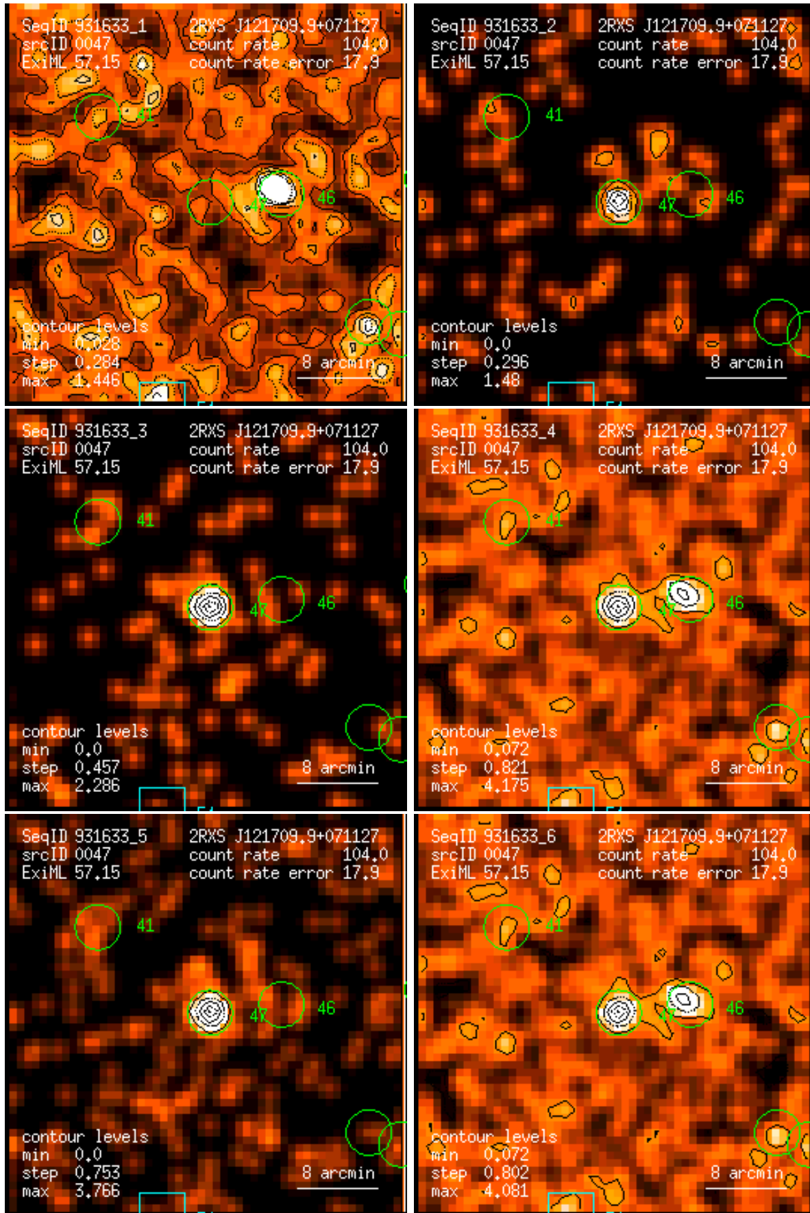
Figure 47: RASS 931633: detection 0047: band rate images, Gaussian filter: (1) PSPC channels 11 – 41, (2) 52 – 90, (3) 91 – 201, (4) 11 – 235, (5) 52 – 201, (6) 11 – 201. Broad band rates in counts/ks. Band rate contour levels in counts/ks/arcmin 2 .
