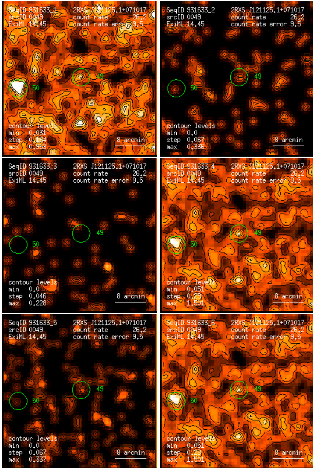
Figure 49: RASS 931633: detection 0049: band rate images, Gaussian filter: (1) PSPC channels 11 – 41, (2) 52 – 90, (3) 91 – 201, (4) 11 – 235, (5) 52 – 201, (6) 11 – 201. Broad band rates in counts/ks. Band rate contour levels in counts/ks/arcmin 2 .
