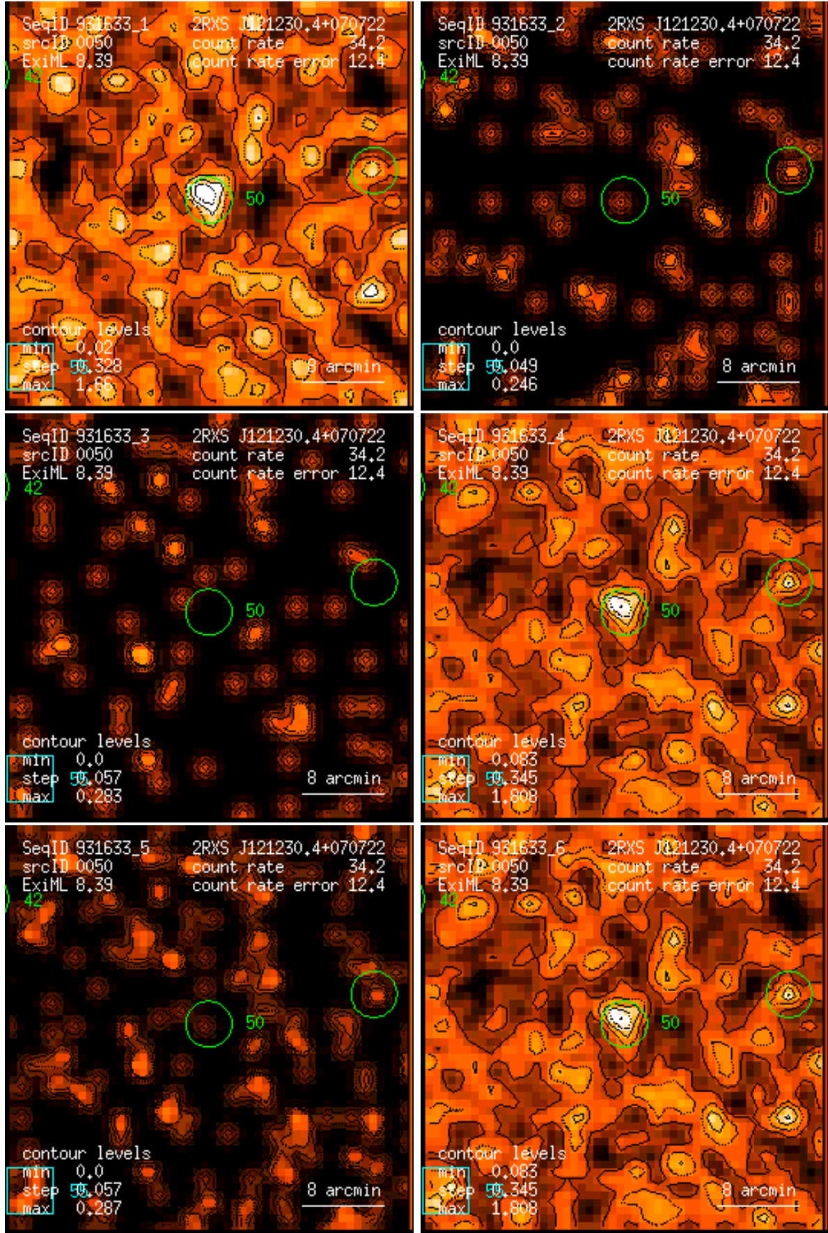
Figure 50: RASS 931633: detection 0050: band rate images, Gaussian filter: (1) PSPC channels 11 – 41, (2) 52 – 90, (3) 91 – 201, (4) 11 – 235, (5) 52 – 201, (6) 11 – 201. Broad band rates in counts/ks. Band rate contour levels in counts/ks/arcmin 2 .
