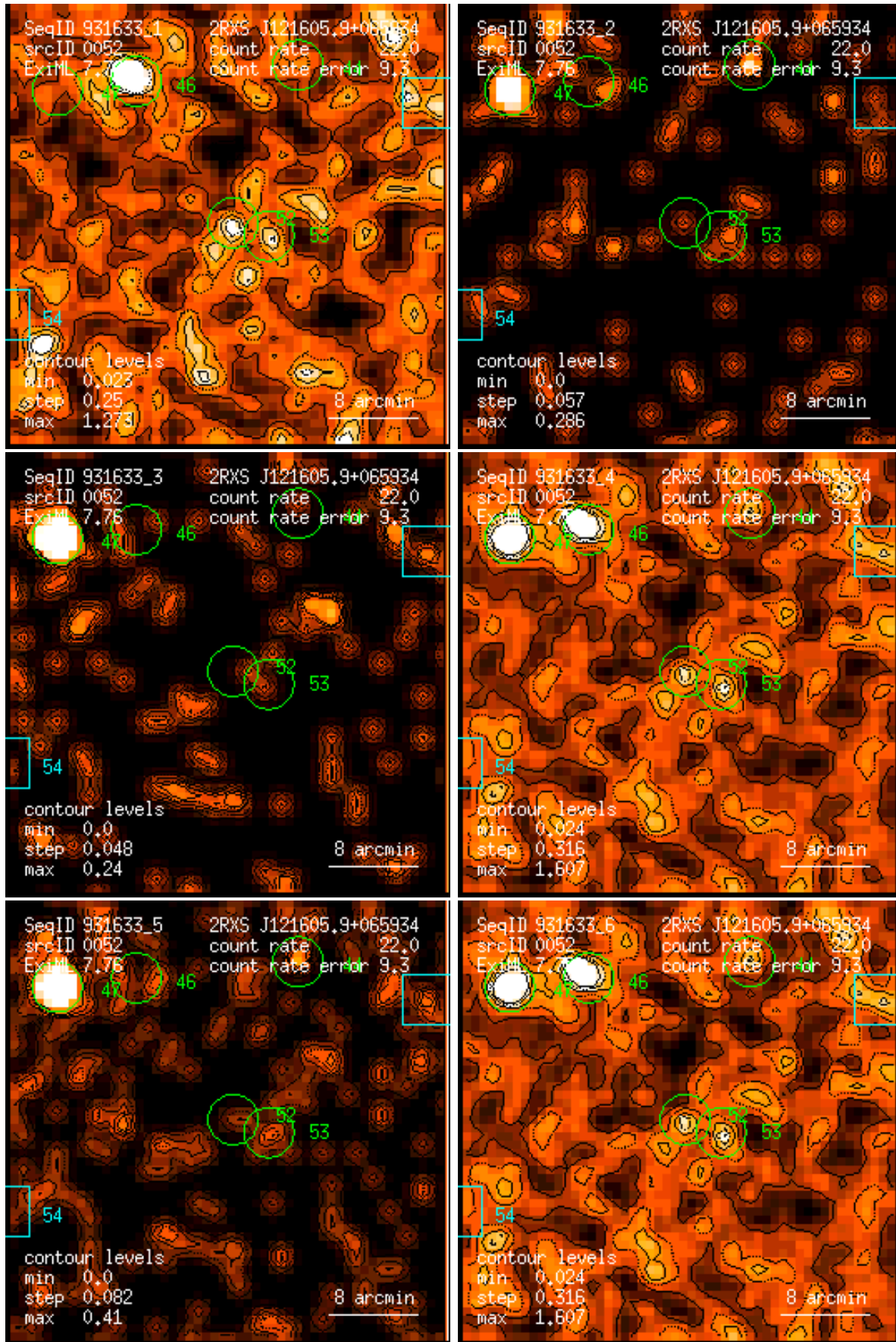
Figure 52: RASS 931633: detection 0052: band rate images, Gaussian filter: (1) PSPC channels 11 – 41, (2) 52 – 90, (3) 91 – 201, (4) 11 – 235, (5) 52 – 201, (6) 11 – 201. Broad band rates in counts/ks. Band rate contour levels in counts/ks/arcmin 2 .
