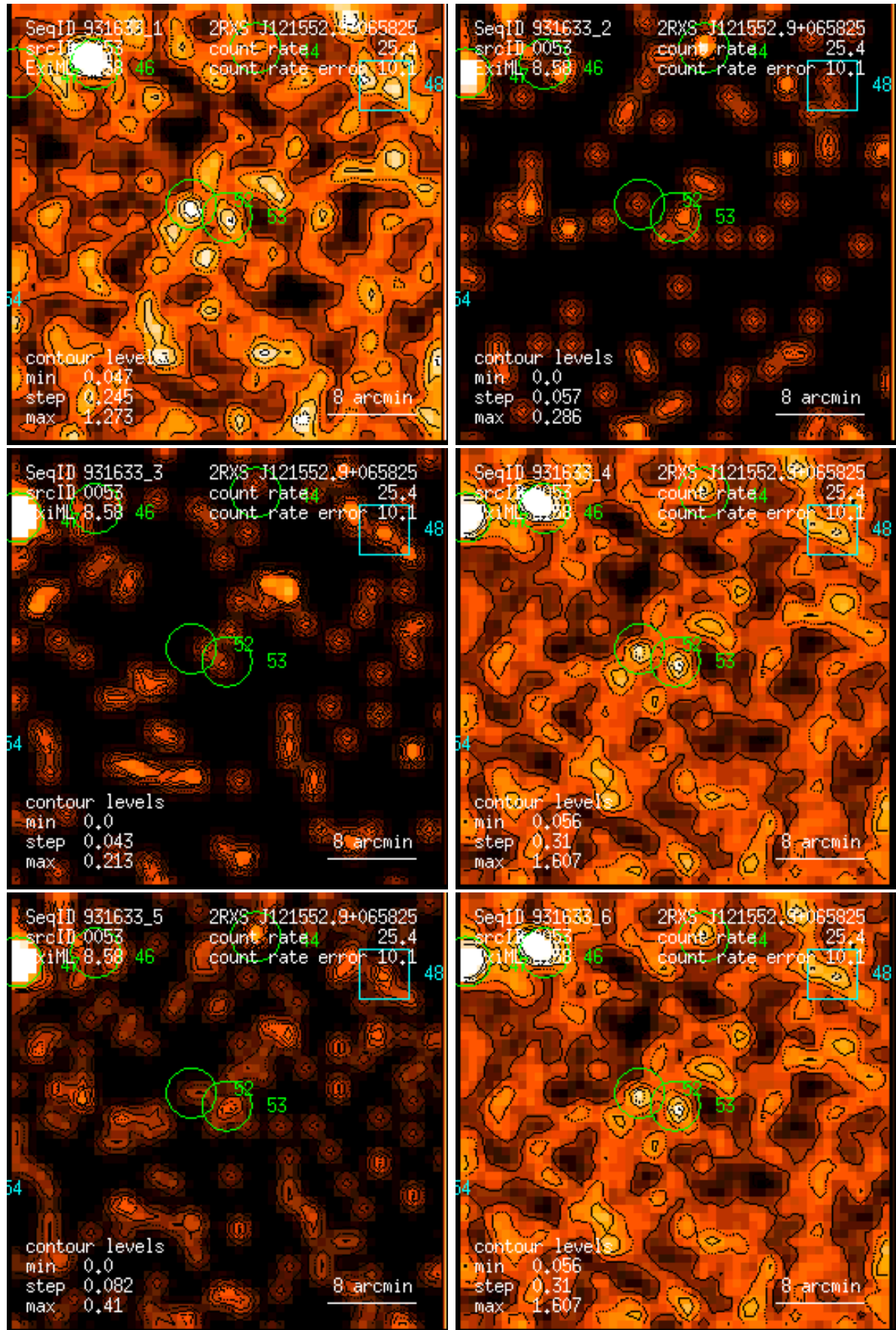
Figure 53: RASS 931633: detection 0053: band rate images, Gaussian filter: (1) PSPC channels 11 – 41, (2) 52 – 90, (3) 91 – 201, (4) 11 – 235, (5) 52 – 201, (6) 11 – 201. Broad band rates in counts/ks. Band rate contour levels in counts/ks/arcmin 2 .
