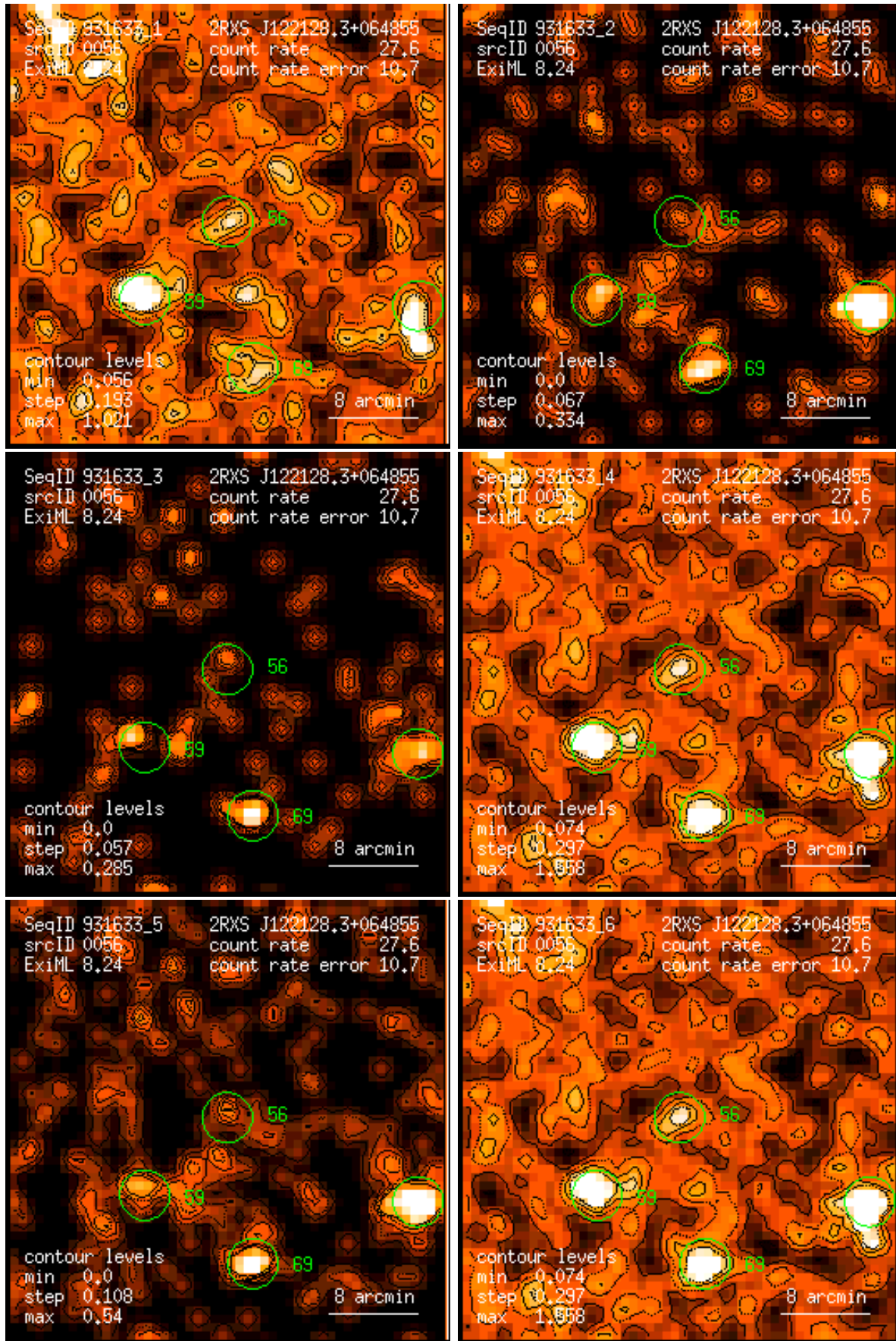
Figure 56: RASS 931633: detection 0056: band rate images, Gaussian filter: (1) PSPC channels 11 – 41, (2) 52 – 90, (3) 91 – 201, (4) 11 – 235, (5) 52 – 201, (6) 11 – 201. Broad band rates in counts/ks. Band rate contour levels in counts/ks/arcmin 2 .
