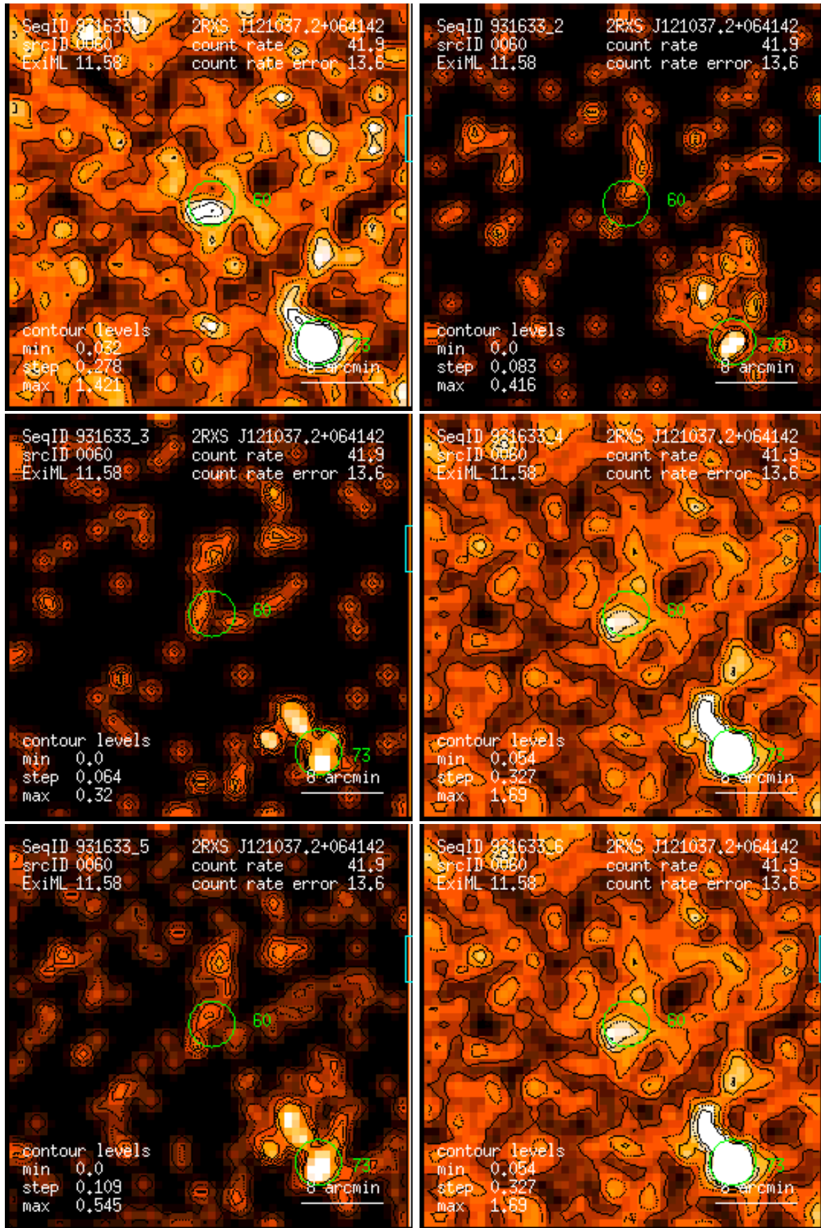
Figure 60: RASS 931633: detection 0060: band rate images, Gaussian filter: (1) PSPC channels 11 – 41, (2) 52 – 90, (3) 91 – 201, (4) 11 – 235, (5) 52 – 201, (6) 11 – 201. Broad band rates in counts/ks. Band rate contour levels in counts/ks/arcmin 2 .
