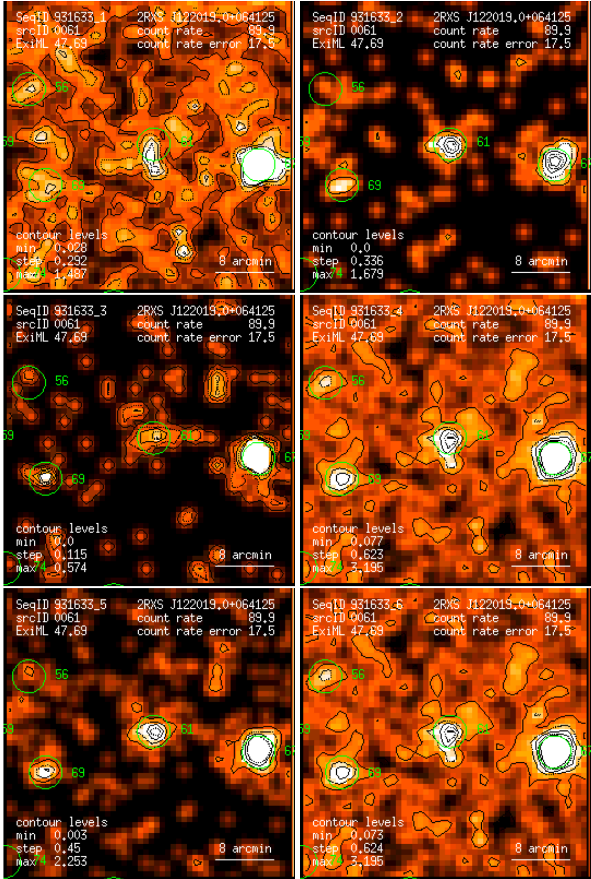
Figure 61: RASS 931633: detection 0061: band rate images, Gaussian filter: (1) PSPC channels 11 – 41, (2) 52 – 90, (3) 91 – 201, (4) 11 – 235, (5) 52 – 201, (6) 11 – 201. Broad band rates in counts/ks. Band rate contour levels in counts/ks/arcmin 2 .
