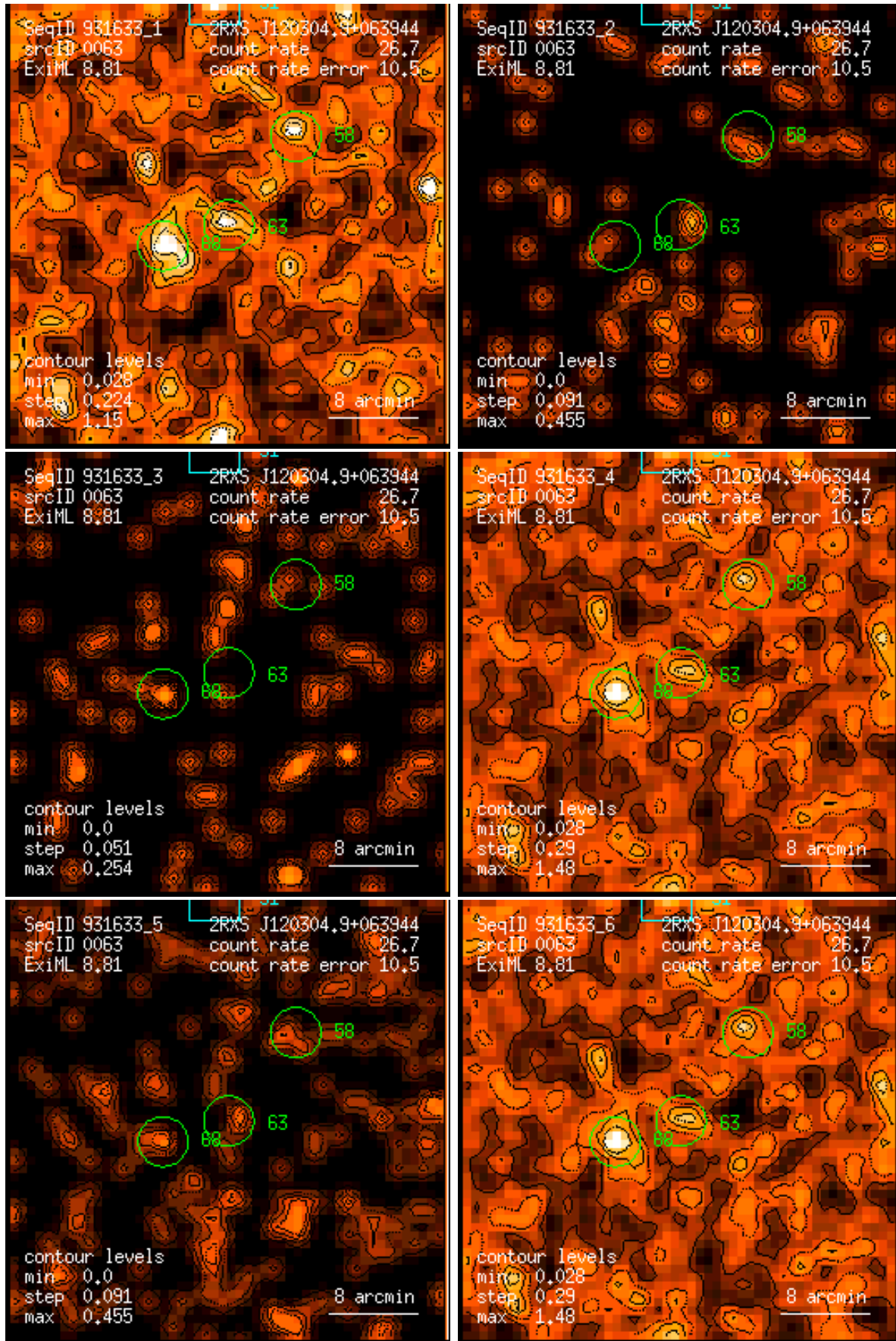
Figure 63: RASS 931633: detection 0063: band rate images, Gaussian filter: (1) PSPC channels 11 – 41, (2) 52 – 90, (3) 91 – 201, (4) 11 – 235, (5) 52 – 201, (6) 11 – 201. Broad band rates in counts/ks. Band rate contour levels in counts/ks/arcmin 2 .
