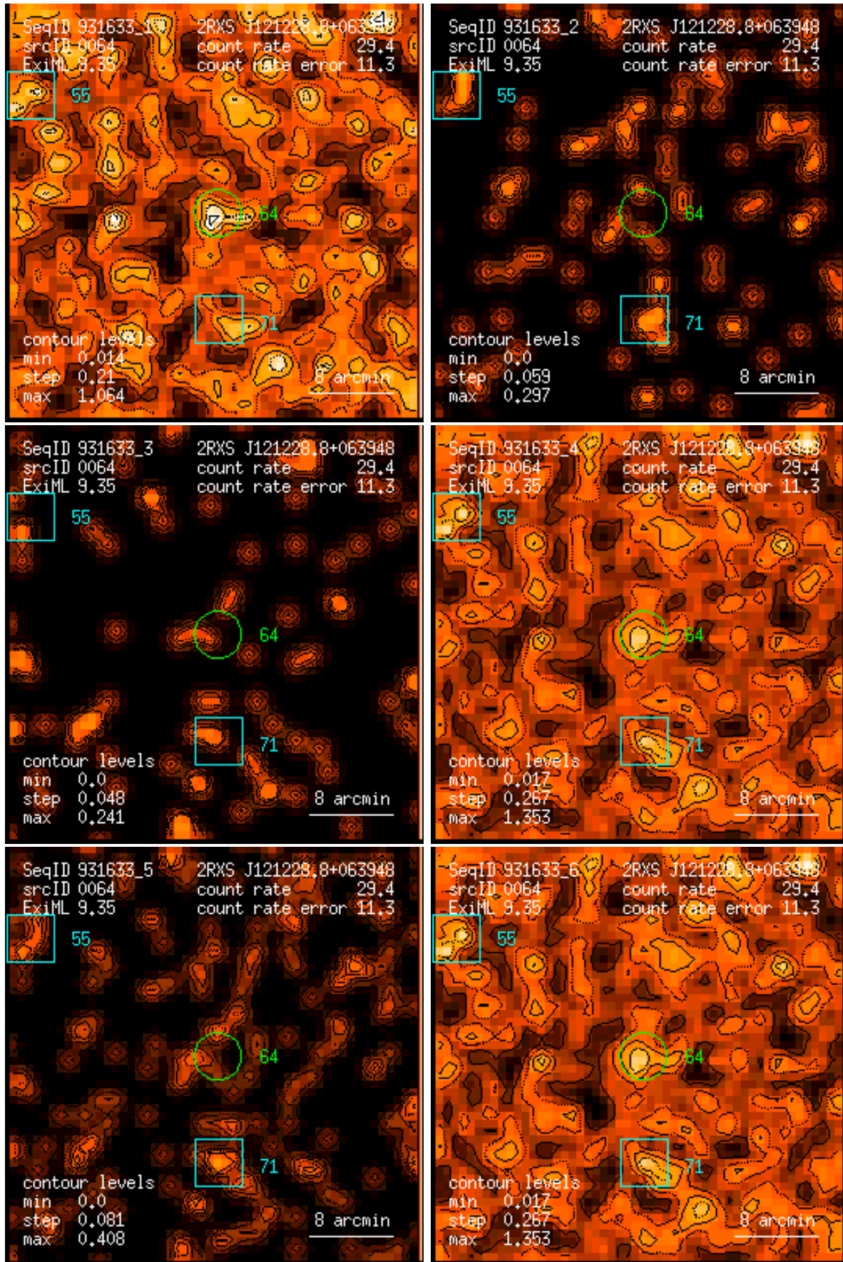
Figure 64: RASS 931633: detection 0064: band rate images, Gaussian filter: (1) PSPC channels 11 – 41, (2) 52 – 90, (3) 91 – 201, (4) 11 – 235, (5) 52 – 201, (6) 11 – 201. Broad band rates in counts/ks. Band rate contour levels in counts/ks/arcmin 2 .
