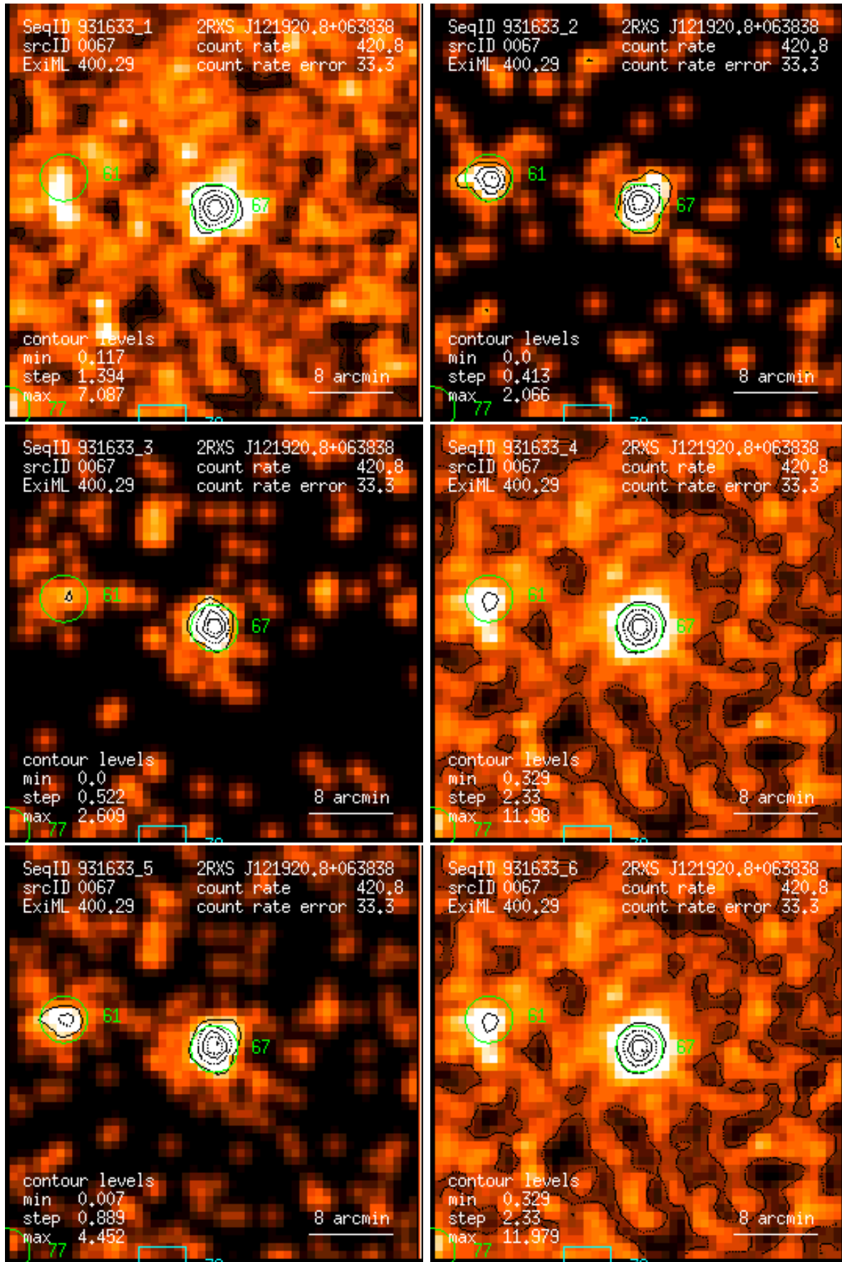
Figure 67: RASS 931633: detection 0067: band rate images, Gaussian filter: (1) PSPC channels 11 – 41, (2) 52 – 90, (3) 91 – 201, (4) 11 – 235, (5) 52 – 201, (6) 11 – 201. Broad band rates in counts/ks. Band rate contour levels in counts/ks/arcmin 2 .
