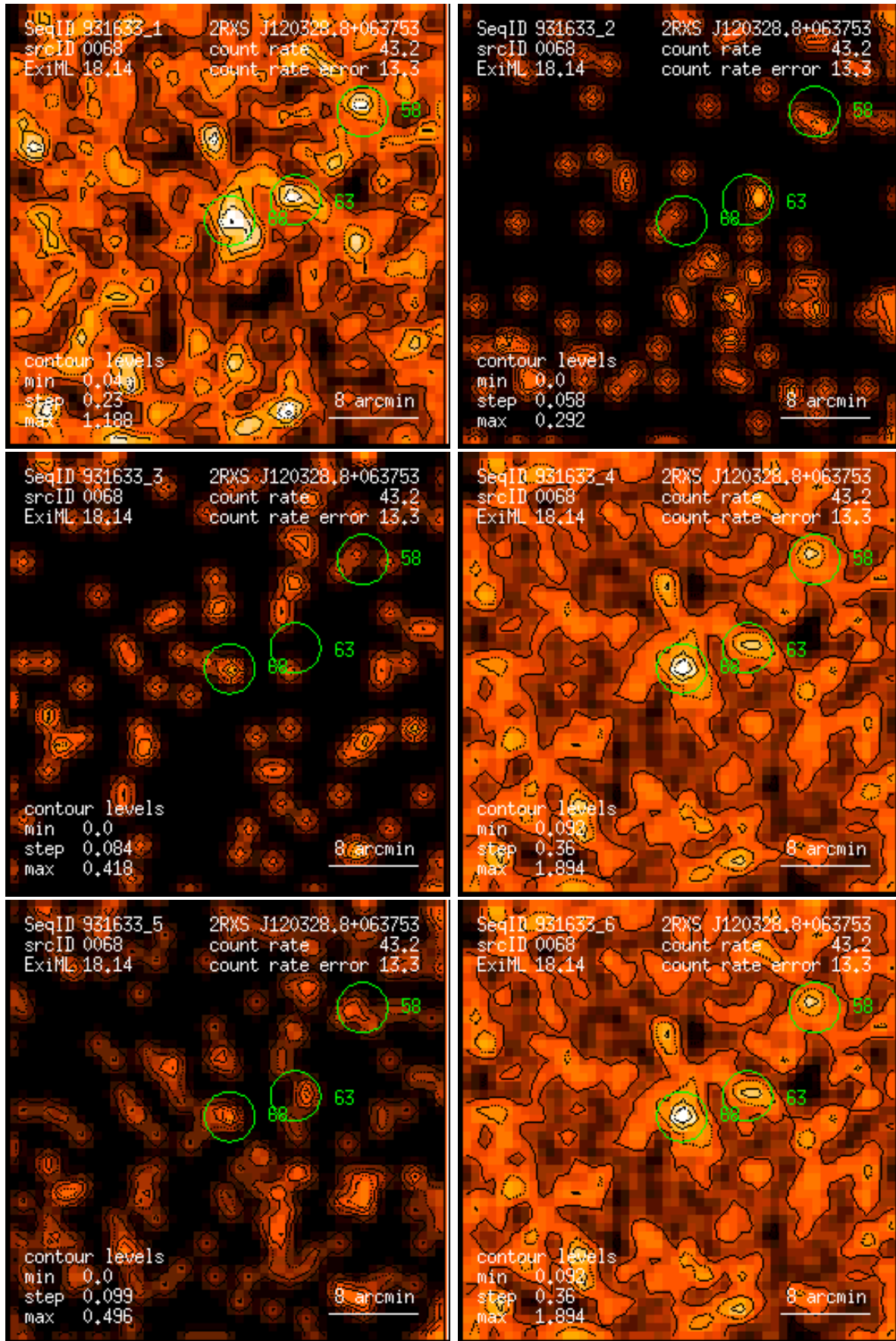
Figure 68: RASS 931633: detection 0068: band rate images, Gaussian filter: (1) PSPC channels 11 – 41, (2) 52 – 90, (3) 91 – 201, (4) 11 – 235, (5) 52 – 201, (6) 11 – 201. Broad band rates in counts/ks. Band rate contour levels in counts/ks/arcmin 2 .
