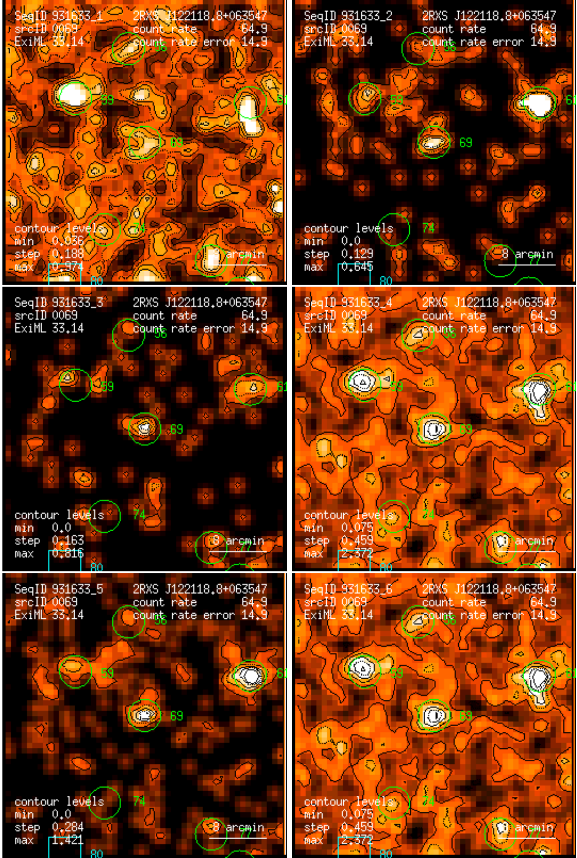
Figure 69: RASS 931633: detection 0069: band rate images, Gaussian filter: (1) PSPC channels 11 – 41, (2) 52 – 90, (3) 91 – 201, (4) 11 – 235, (5) 52 – 201, (6) 11 – 201. Broad band rates in counts/ks. Band rate contour levels in counts/ks/arcmin 2 .
