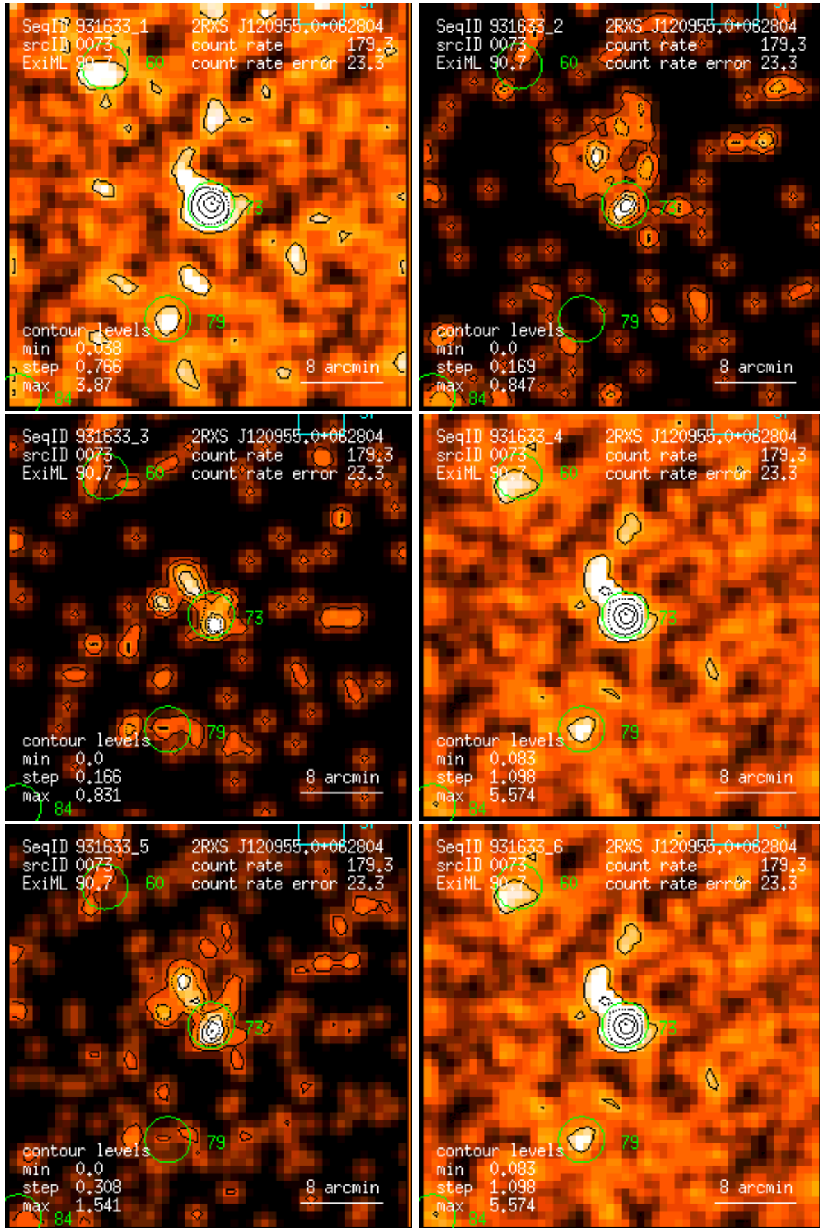
Figure 73: RASS 931633: detection 0073: band rate images, Gaussian filter: (1) PSPC channels 11 – 41, (2) 52 – 90, (3) 91 – 201, (4) 11 – 235, (5) 52 – 201, (6) 11 – 201. Broad band rates in counts/ks. Band rate contour levels in counts/ks/arcmin 2 .
