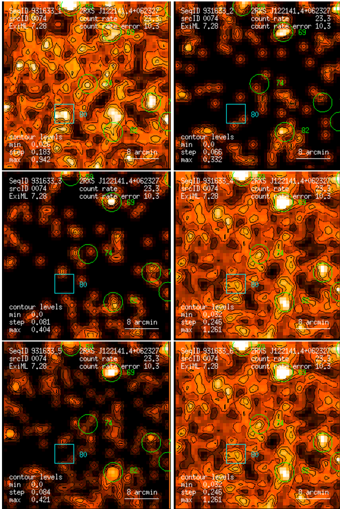
Figure 74: RASS 931633: detection 0074: band rate images, Gaussian filter: (1) PSPC channels 11 – 41, (2) 52 – 90, (3) 91 – 201, (4) 11 – 235, (5) 52 – 201, (6) 11 – 201. Broad band rates in counts/ks. Band rate contour levels in counts/ks/arcmin 2 .
