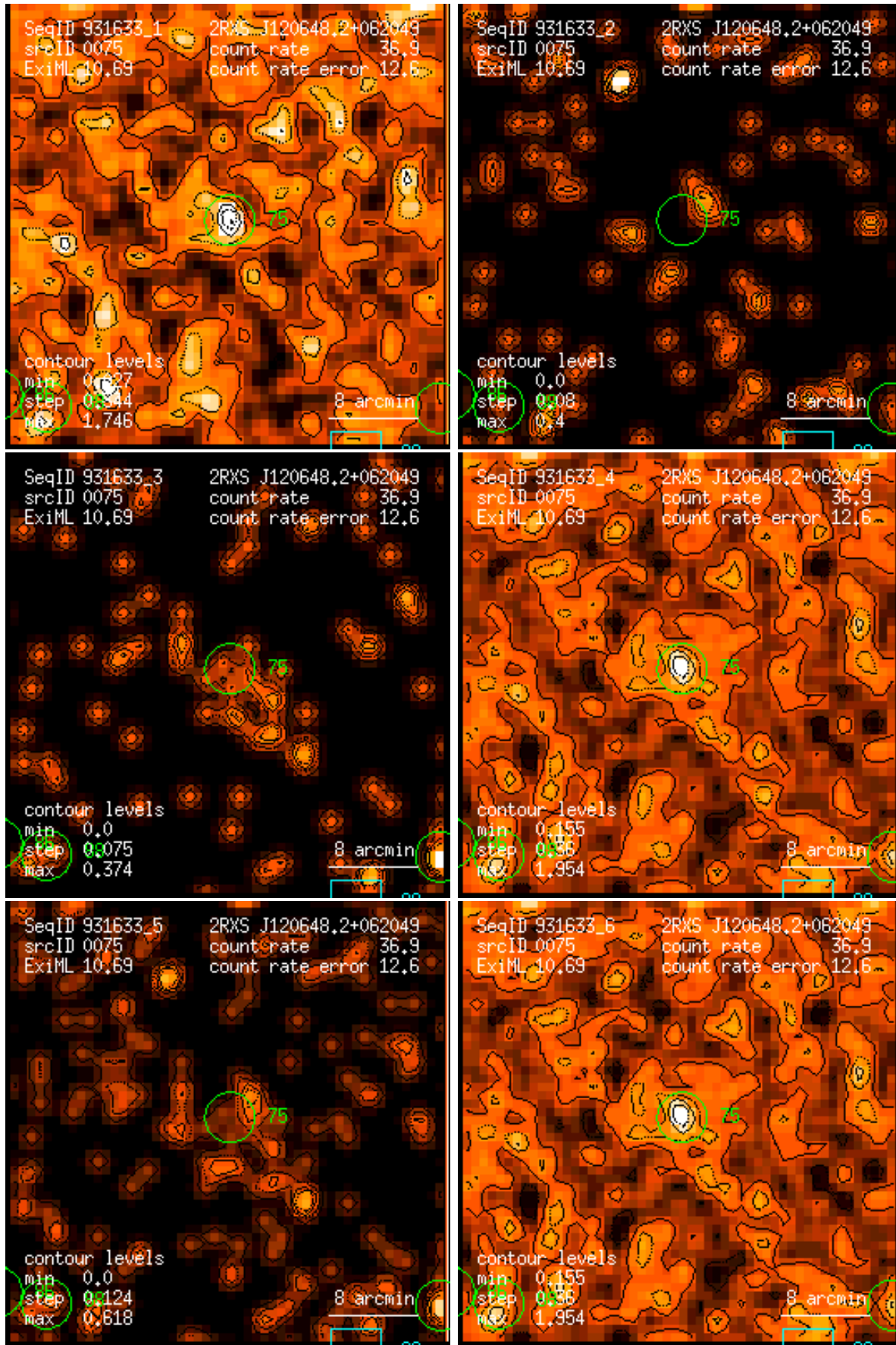
Figure 75: RASS 931633: detection 0075: band rate images, Gaussian filter: (1) PSPC channels 11 – 41, (2) 52 – 90, (3) 91 – 201, (4) 11 – 235, (5) 52 – 201, (6) 11 – 201. Broad band rates in counts/ks. Band rate contour levels in counts/ks/arcmin 2 .
