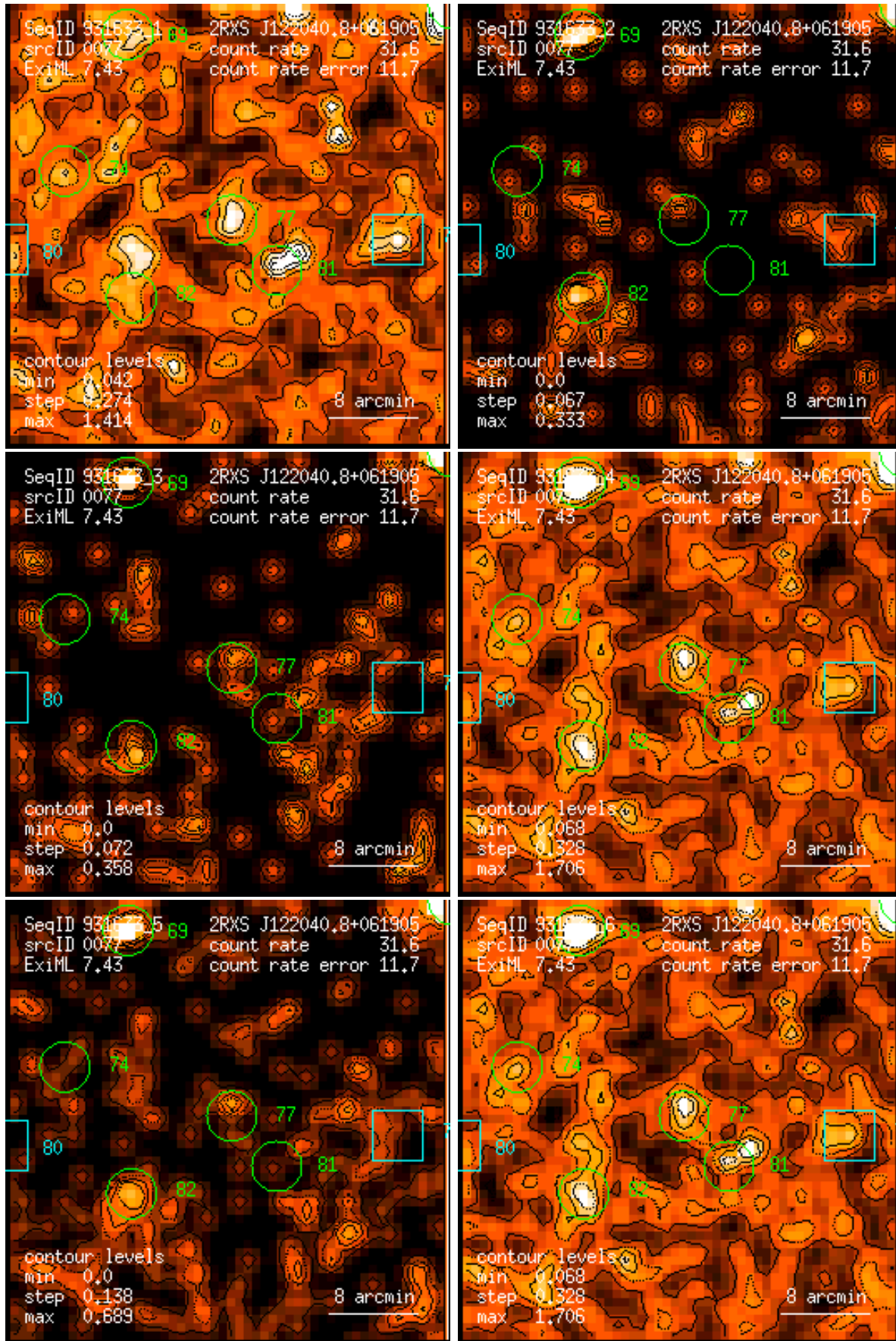
Figure 77: RASS 931633: detection 0077: band rate images, Gaussian filter: (1) PSPC channels 11 – 41, (2) 52 – 90, (3) 91 – 201, (4) 11 – 235, (5) 52 – 201, (6) 11 – 201. Broad band rates in counts/ks. Band rate contour levels in counts/ks/arcmin 2 .
