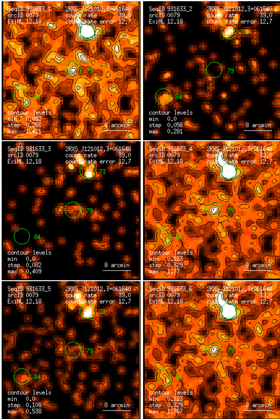
Figure 79: RASS 931633: detection 0079: band rate images, Gaussian filter: (1) PSPC channels 11 – 41, (2) 52 – 90, (3) 91 – 201, (4) 11 – 235, (5) 52 – 201, (6) 11 – 201. Broad band rates in counts/ks. Band rate contour levels in counts/ks/arcmin 2 .
