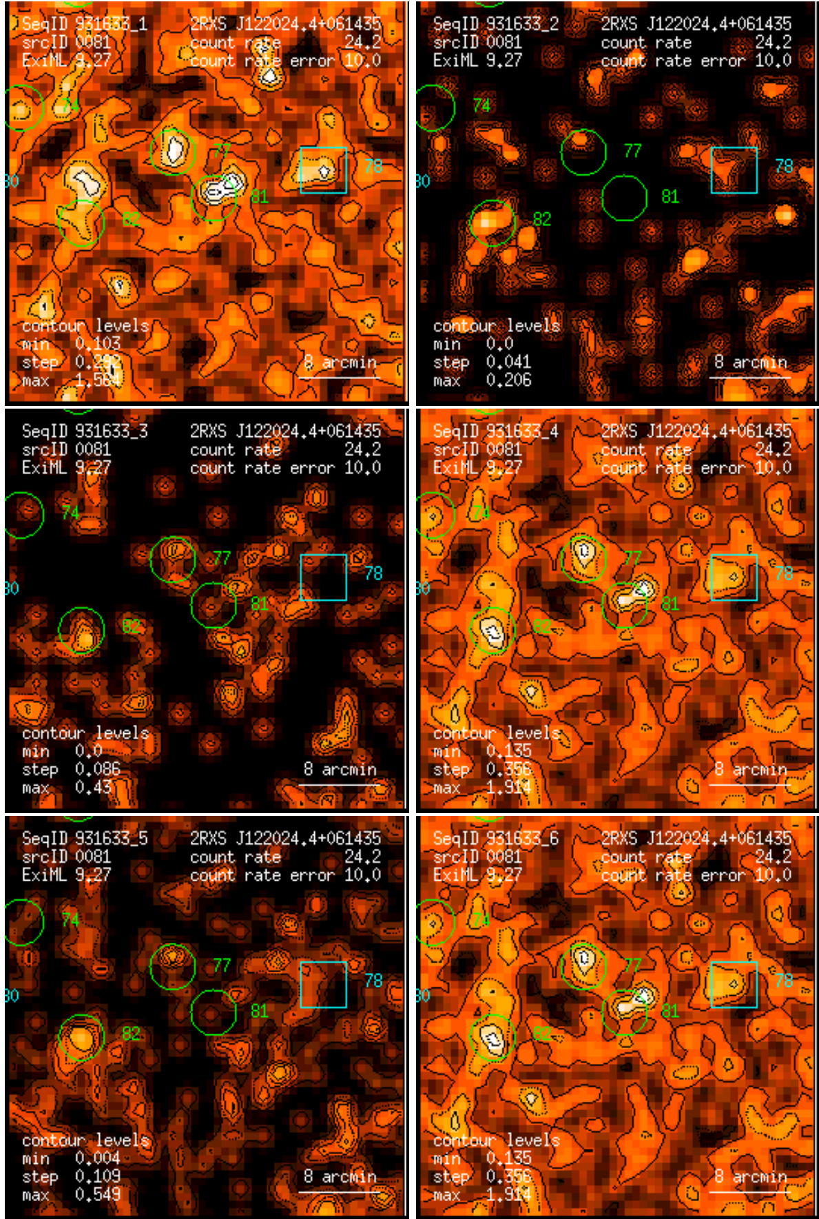
Figure 81: RASS 931633: detection 0081: band rate images, Gaussian filter: (1) PSPC channels 11 – 41, (2) 52 – 90, (3) 91 – 201, (4) 11 – 235, (5) 52 – 201, (6) 11 – 201. Broad band rates in counts/ks. Band rate contour levels in counts/ks/arcmin 2 .
