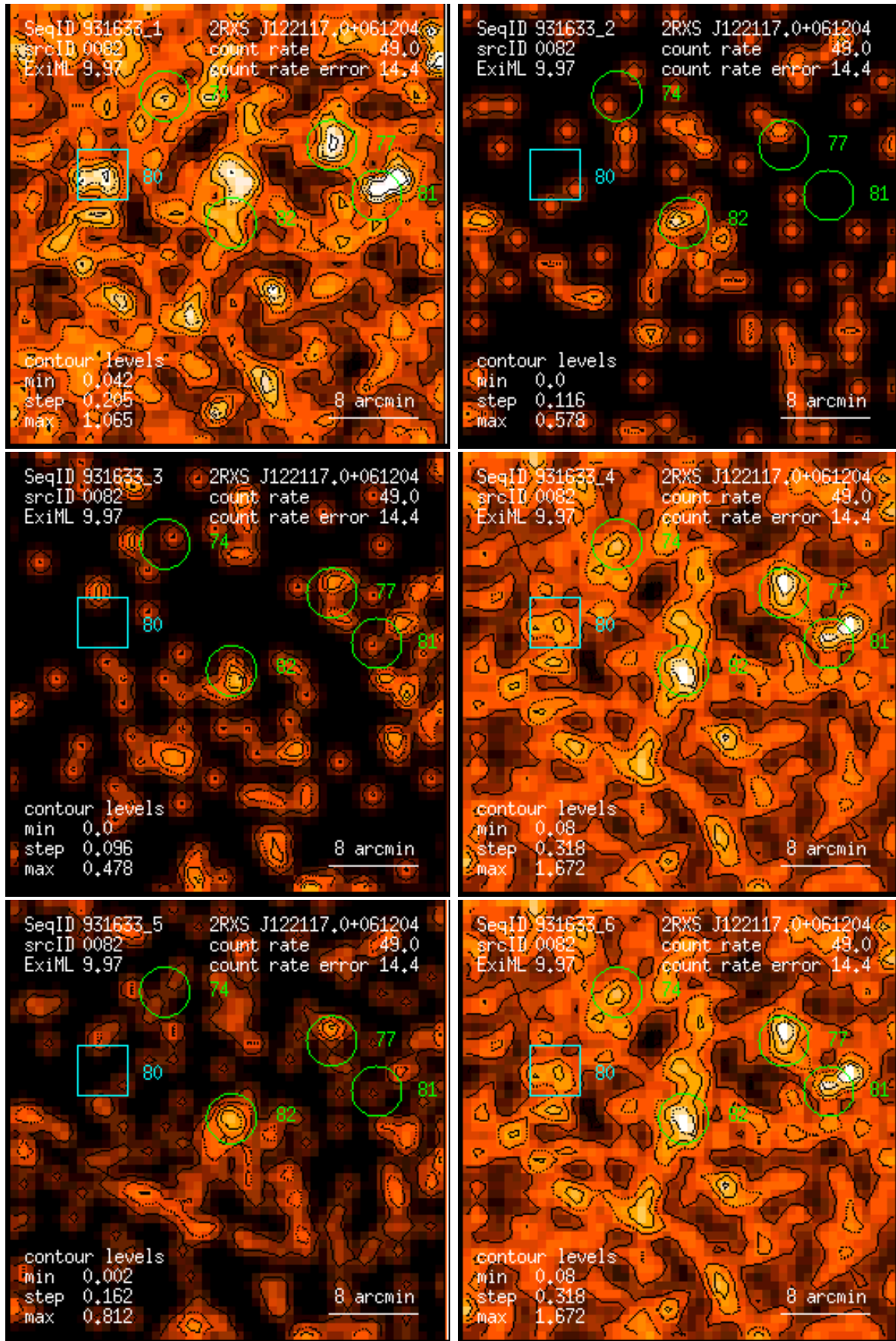
Figure 82: RASS 931633: detection 0082: band rate images, Gaussian filter: (1) PSPC channels 11 – 41, (2) 52 – 90, (3) 91 – 201, (4) 11 – 235, (5) 52 – 201, (6) 11 – 201. Broad band rates in counts/ks. Band rate contour levels in counts/ks/arcmin 2 .
