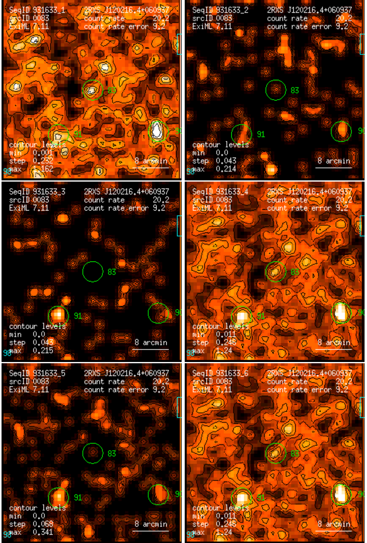
Figure 83: RASS 931633: detection 0083: band rate images, Gaussian filter: (1) PSPC channels 11 – 41, (2) 52 – 90, (3) 91 – 201, (4) 11 – 235, (5) 52 – 201, (6) 11 – 201. Broad band rates in counts/ks. Band rate contour levels in counts/ks/arcmin 2 .
