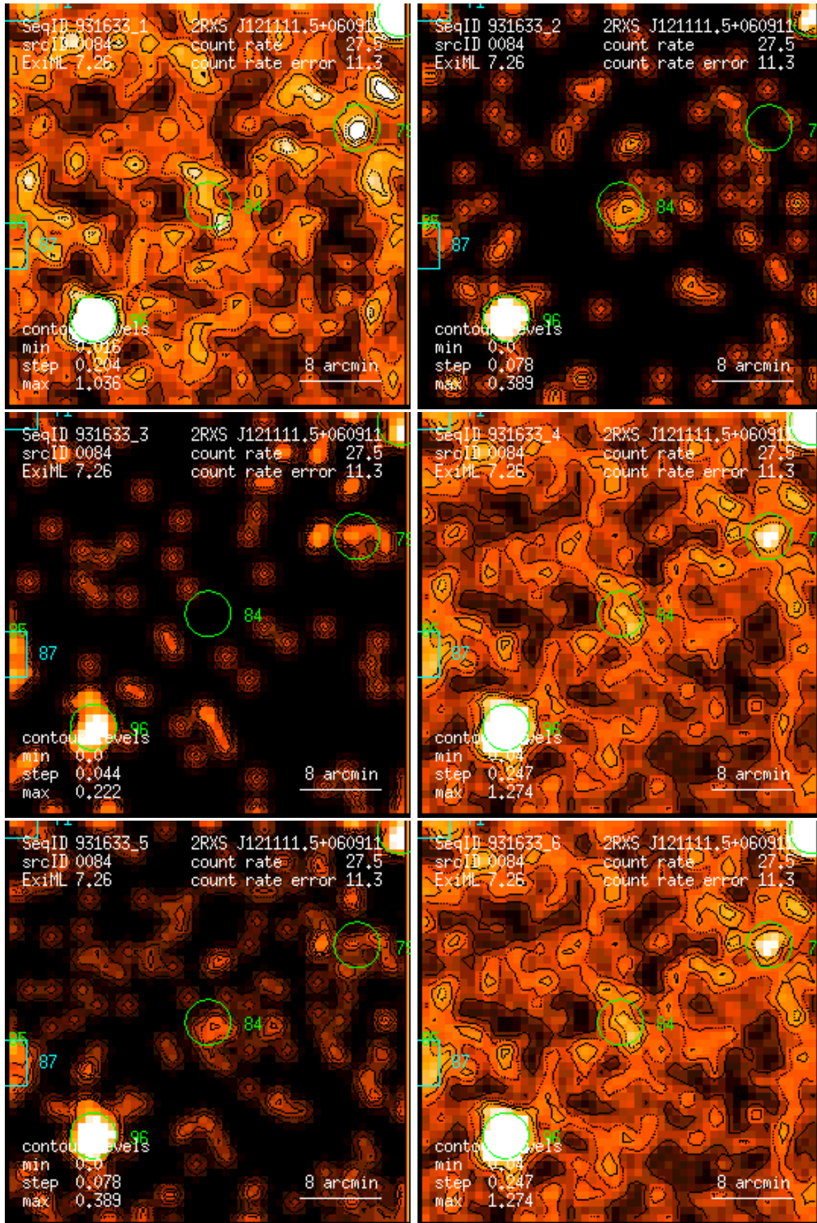
Figure 84: RASS 931633: detection 0084: band rate images, Gaussian filter: (1) PSPC channels 11 – 41, (2) 52 – 90, (3) 91 – 201, (4) 11 – 235, (5) 52 – 201, (6) 11 – 201. Broad band rates in counts/ks. Band rate contour levels in counts/ks/arcmin 2 .
