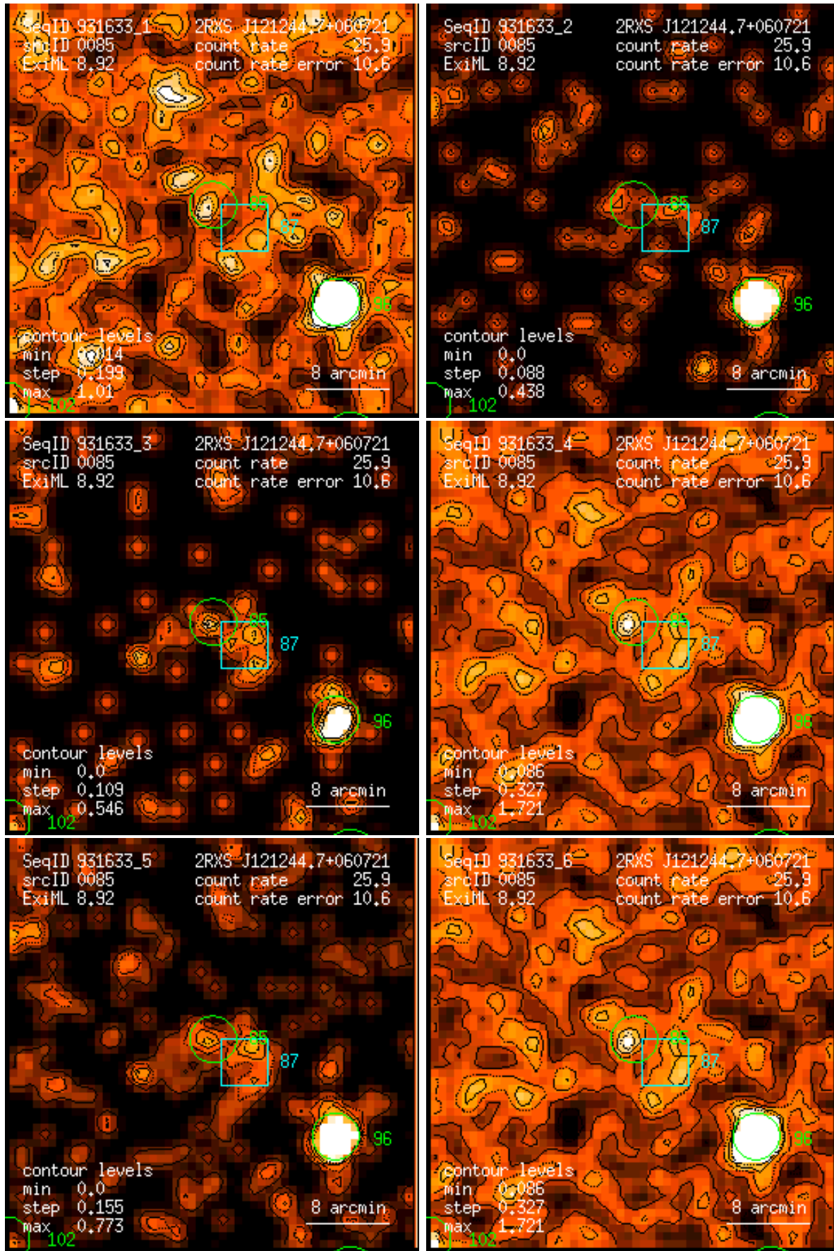
Figure 85: RASS 931633: detection 0085: band rate images, Gaussian filter: (1) PSPC channels 11 – 41, (2) 52 – 90, (3) 91 – 201, (4) 11 – 235, (5) 52 – 201, (6) 11 – 201. Broad band rates in counts/ks. Band rate contour levels in counts/ks/arcmin 2 .
