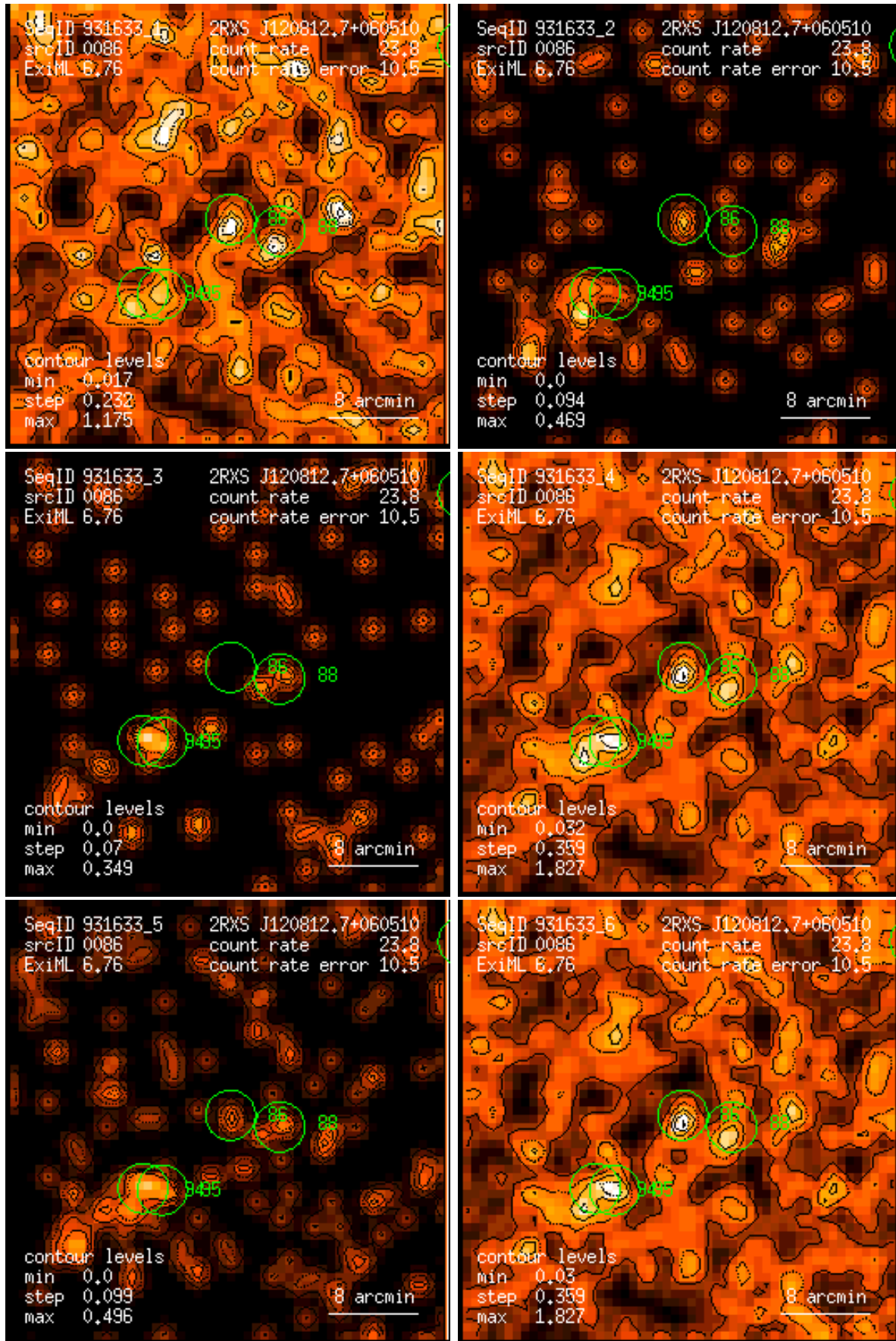
Figure 86: RASS 931633: detection 0086: band rate images, Gaussian filter: (1) PSPC channels 11 – 41, (2) 52 – 90, (3) 91 – 201, (4) 11 – 235, (5) 52 – 201, (6) 11 – 201. Broad band rates in counts/ks. Band rate contour levels in counts/ks/arcmin 2 .
