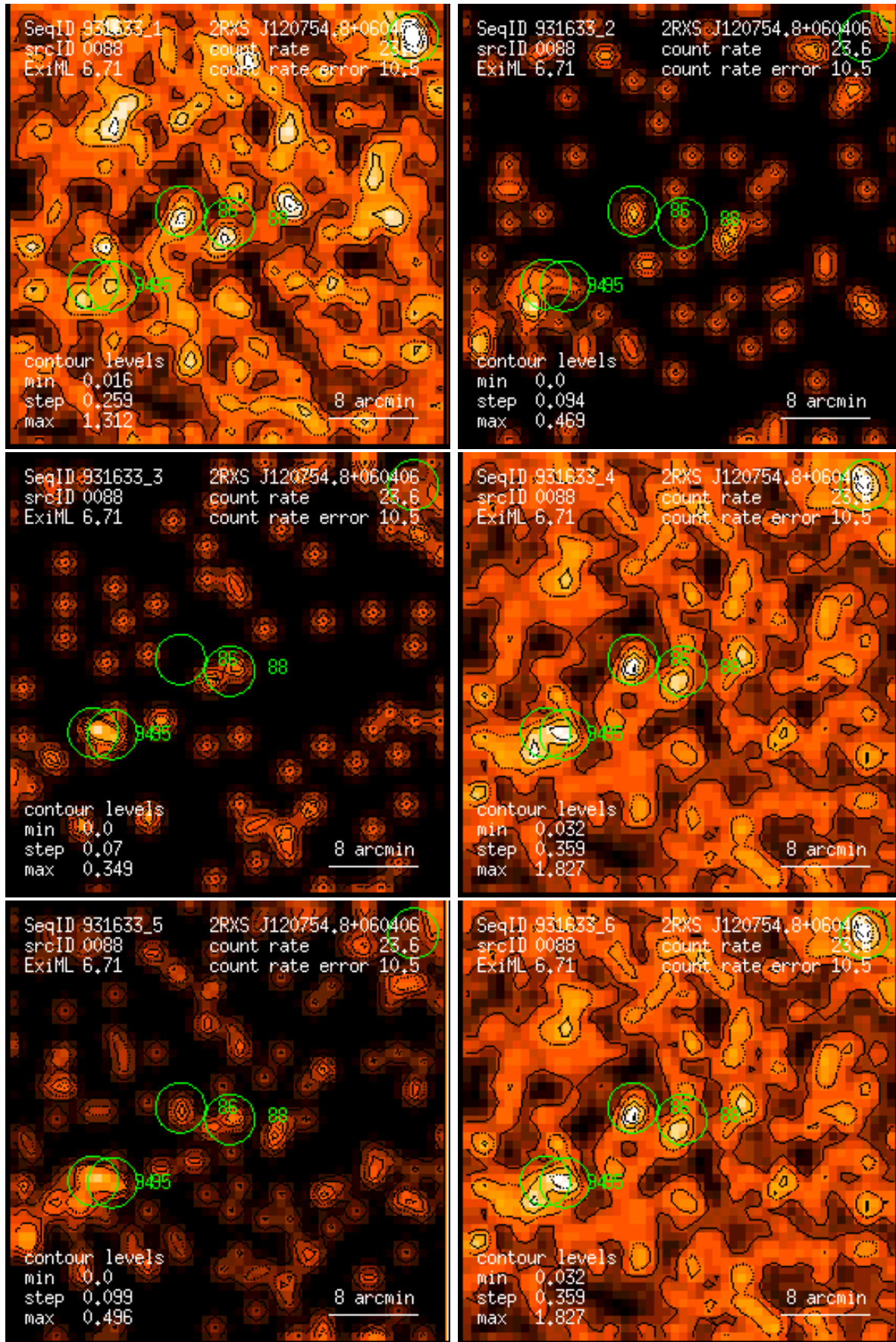
Figure 88: RASS 931633: detection 0088: band rate images, Gaussian filter: (1) PSPC channels 11 – 41, (2) 52 – 90, (3) 91 – 201, (4) 11 – 235, (5) 52 – 201, (6) 11 – 201. Broad band rates in counts/ks. Band rate contour levels in counts/ks/arcmin 2 .
