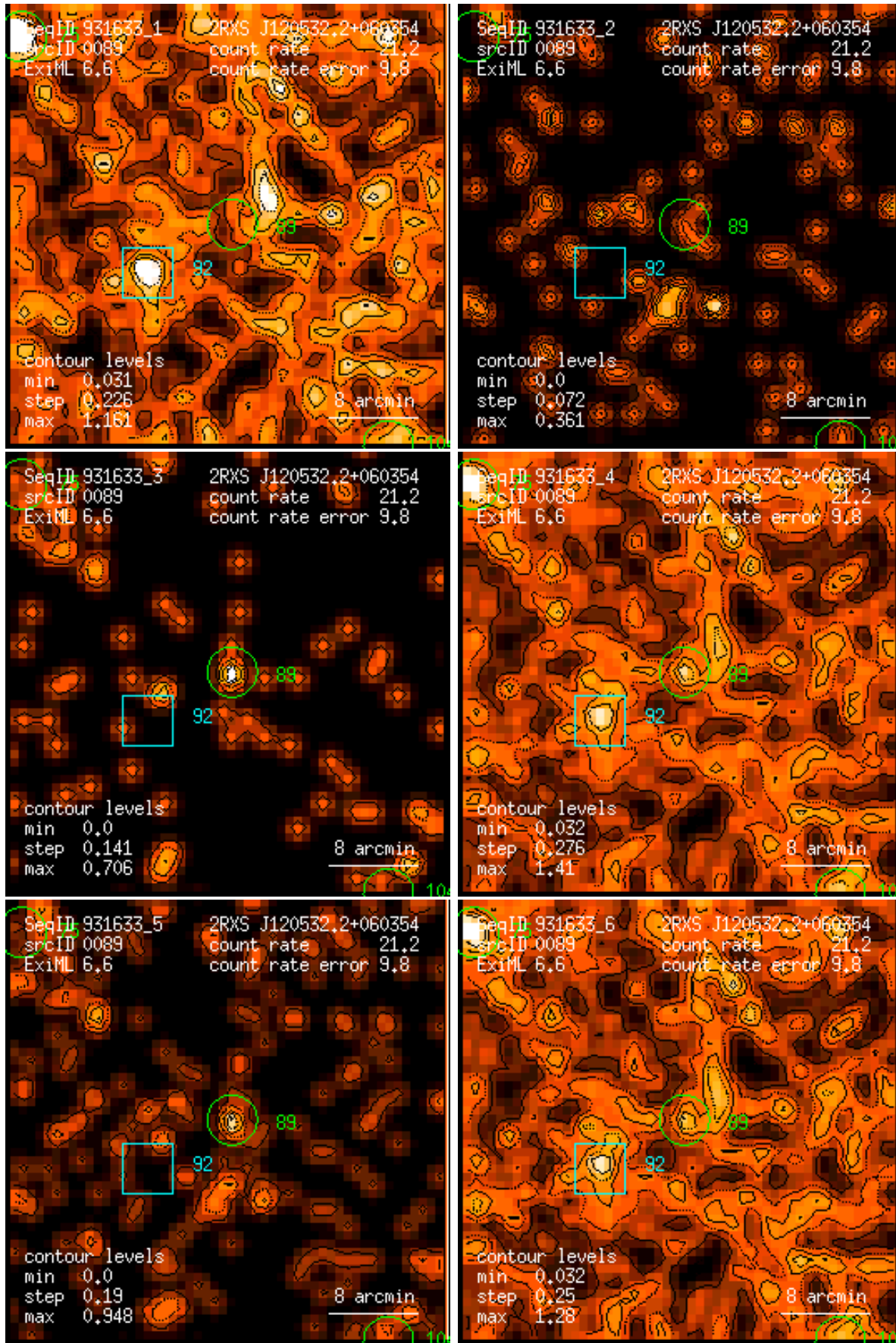
Figure 89: RASS 931633: detection 0089: band rate images, Gaussian filter: (1) PSPC channels 11 – 41, (2) 52 – 90, (3) 91 – 201, (4) 11 – 235, (5) 52 – 201, (6) 11 – 201. Broad band rates in counts/ks. Band rate contour levels in counts/ks/arcmin 2 .
