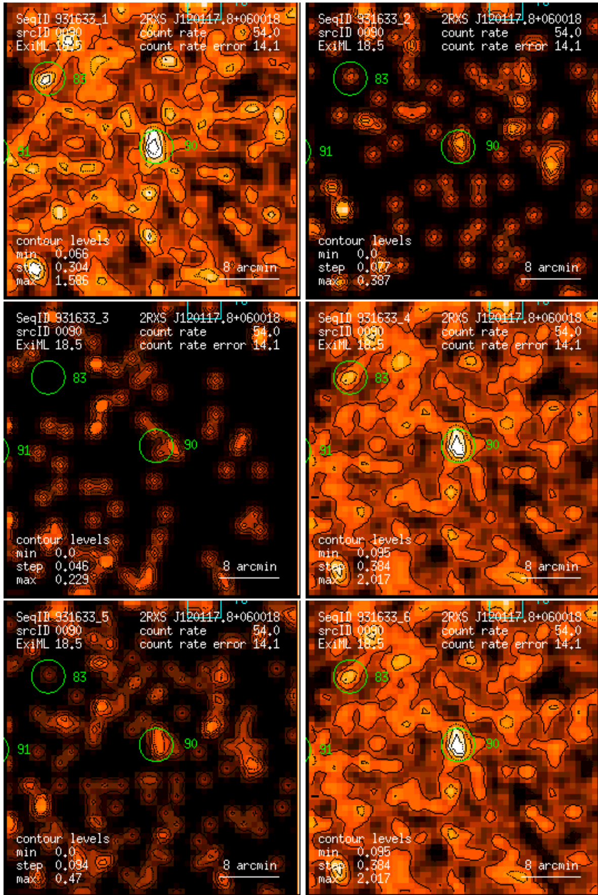
Figure 90: RASS 931633: detection 0090: band rate images, Gaussian filter: (1) PSPC channels 11 – 41, (2) 52 – 90, (3) 91 – 201, (4) 11 – 235, (5) 52 – 201, (6) 11 – 201. Broad band rates in counts/ks. Band rate contour levels in counts/ks/arcmin 2 .
