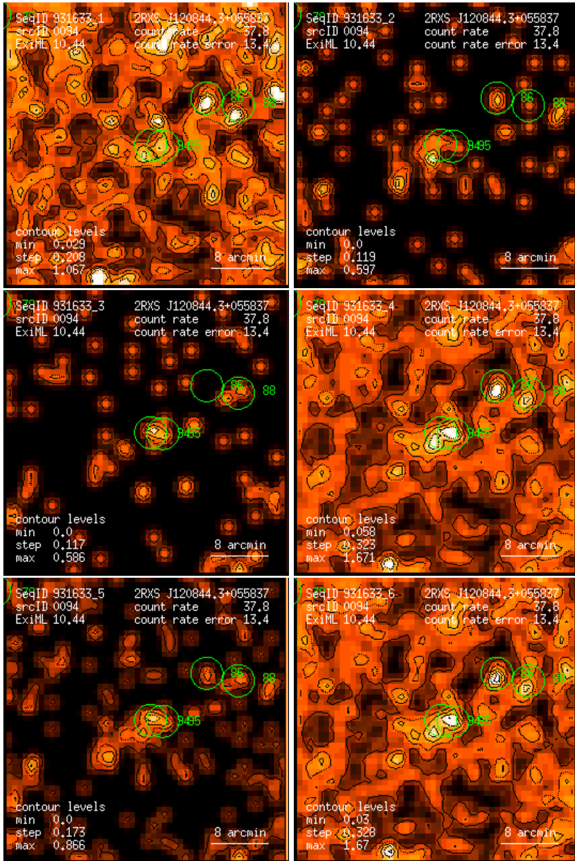
Figure 94: RASS 931633: detection 0094: band rate images, Gaussian filter: (1) PSPC channels 11 – 41, (2) 52 – 90, (3) 91 – 201, (4) 11 – 235, (5) 52 – 201, (6) 11 – 201. Broad band rates in counts/ks. Band rate contour levels in counts/ks/arcmin 2 .
