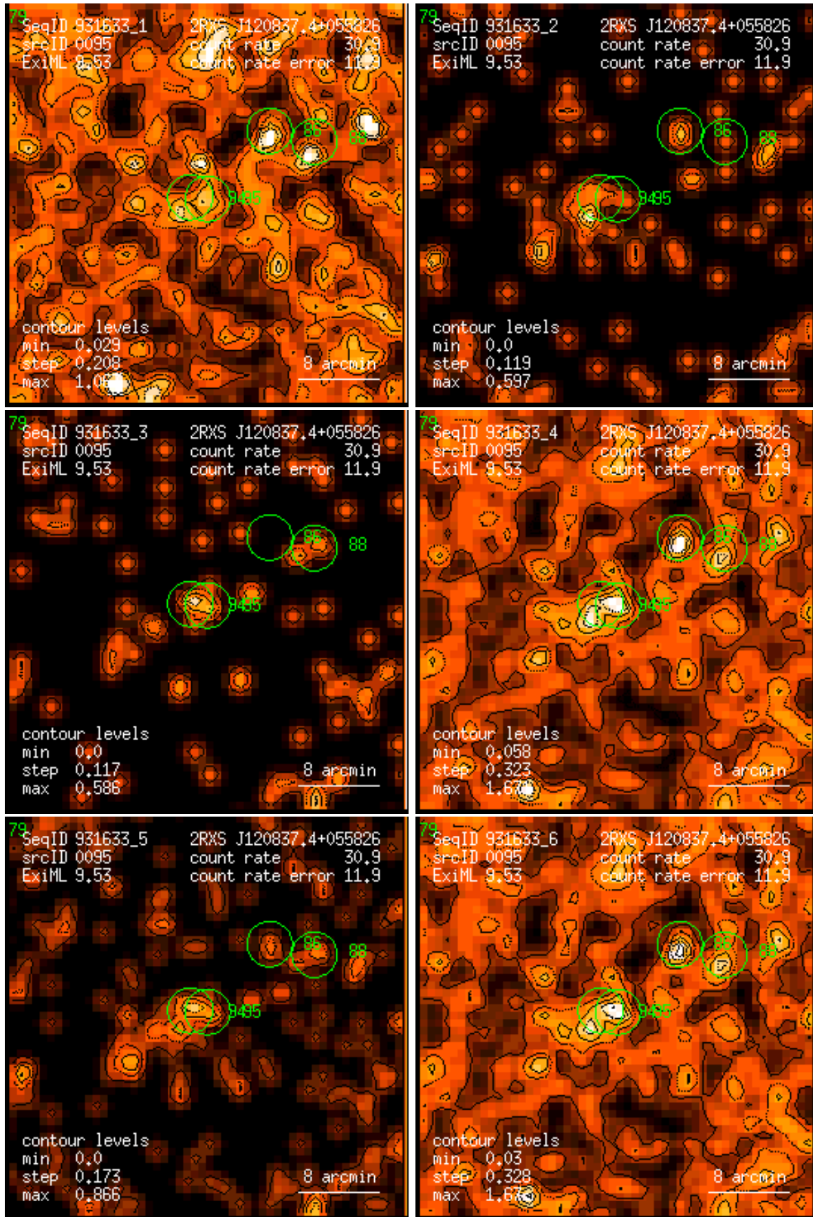
Figure 95: RASS 931633: detection 0095: band rate images, Gaussian filter: (1) PSPC channels 11 – 41, (2) 52 – 90, (3) 91 – 201, (4) 11 – 235, (5) 52 – 201, (6) 11 – 201. Broad band rates in counts/ks. Band rate contour levels in counts/ks/arcmin 2 .
