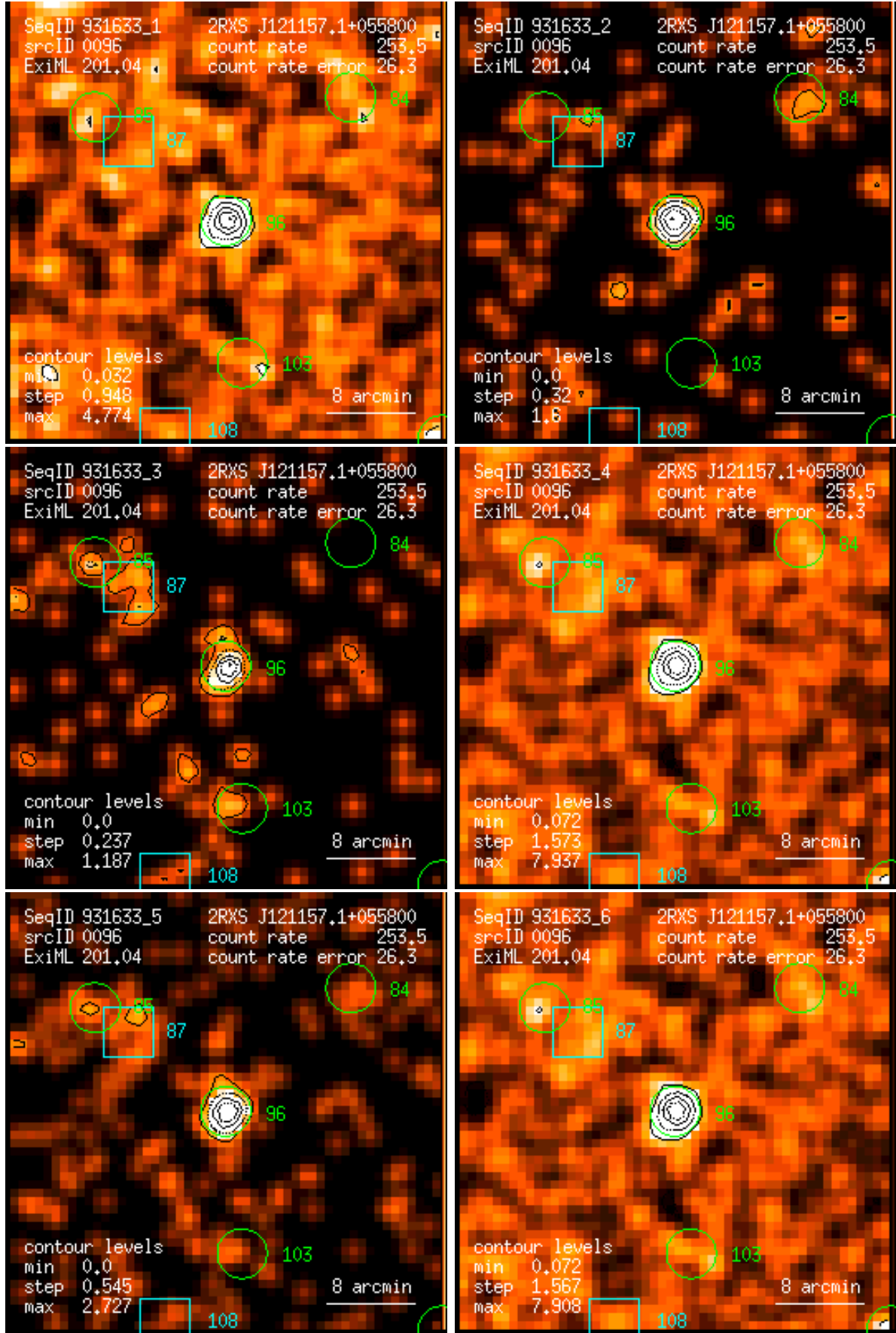
Figure 96: RASS 931633: detection 0096: band rate images, Gaussian filter: (1) PSPC channels 11 – 41, (2) 52 – 90, (3) 91 – 201, (4) 11 – 235, (5) 52 – 201, (6) 11 – 201. Broad band rates in counts/ks. Band rate contour levels in counts/ks/arcmin 2 .
