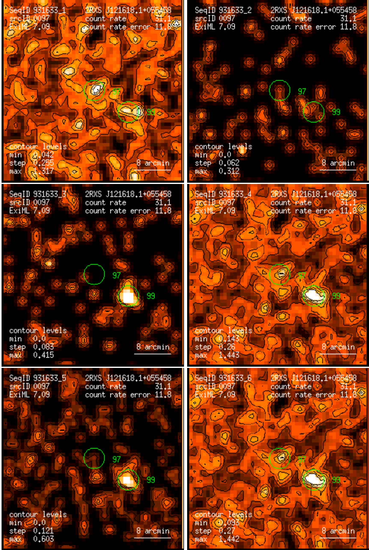
Figure 97: RASS 931633: detection 0097: band rate images, Gaussian filter: (1) PSPC channels 11 – 41, (2) 52 – 90, (3) 91 – 201, (4) 11 – 235, (5) 52 – 201, (6) 11 – 201. Broad band rates in counts/ks. Band rate contour levels in counts/ks/arcmin 2 .
