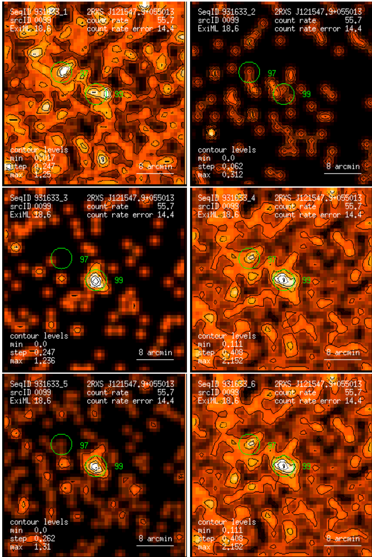
Figure 99: RASS 931633: detection 0099: band rate images, Gaussian filter: (1) PSPC channels 11 – 41, (2) 52 – 90, (3) 91 – 201, (4) 11 – 235, (5) 52 – 201, (6) 11 – 201. Broad band rates in counts/ks. Band rate contour levels in counts/ks/arcmin 2 .
