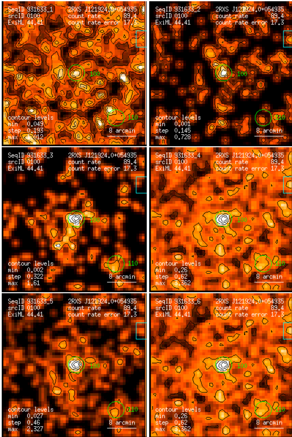
Figure 100: RASS 931633: detection 0100: band rate images, Gaussian filter: (1) PSPC channels 11 – 41, (2) 52 – 90, (3) 91 – 201, (4) 11 – 235, (5) 52 – 201, (6) 11 – 201. Broad band rates in counts/ks. Band rate contour levels in counts/ks/arcmin 2 .
