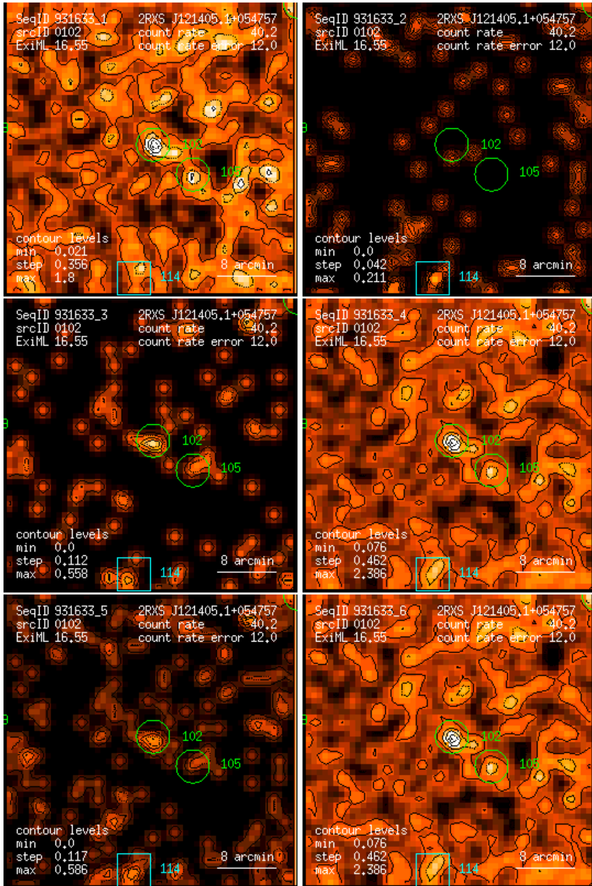
Figure 102: RASS 931633: detection 0102: band rate images, Gaussian filter: (1) PSPC channels 11 – 41, (2) 52 – 90, (3) 91 – 201, (4) 11 – 235, (5) 52 – 201, (6) 11 – 201. Broad band rates in counts/ks. Band rate contour levels in counts/ks/arcmin 2 .
