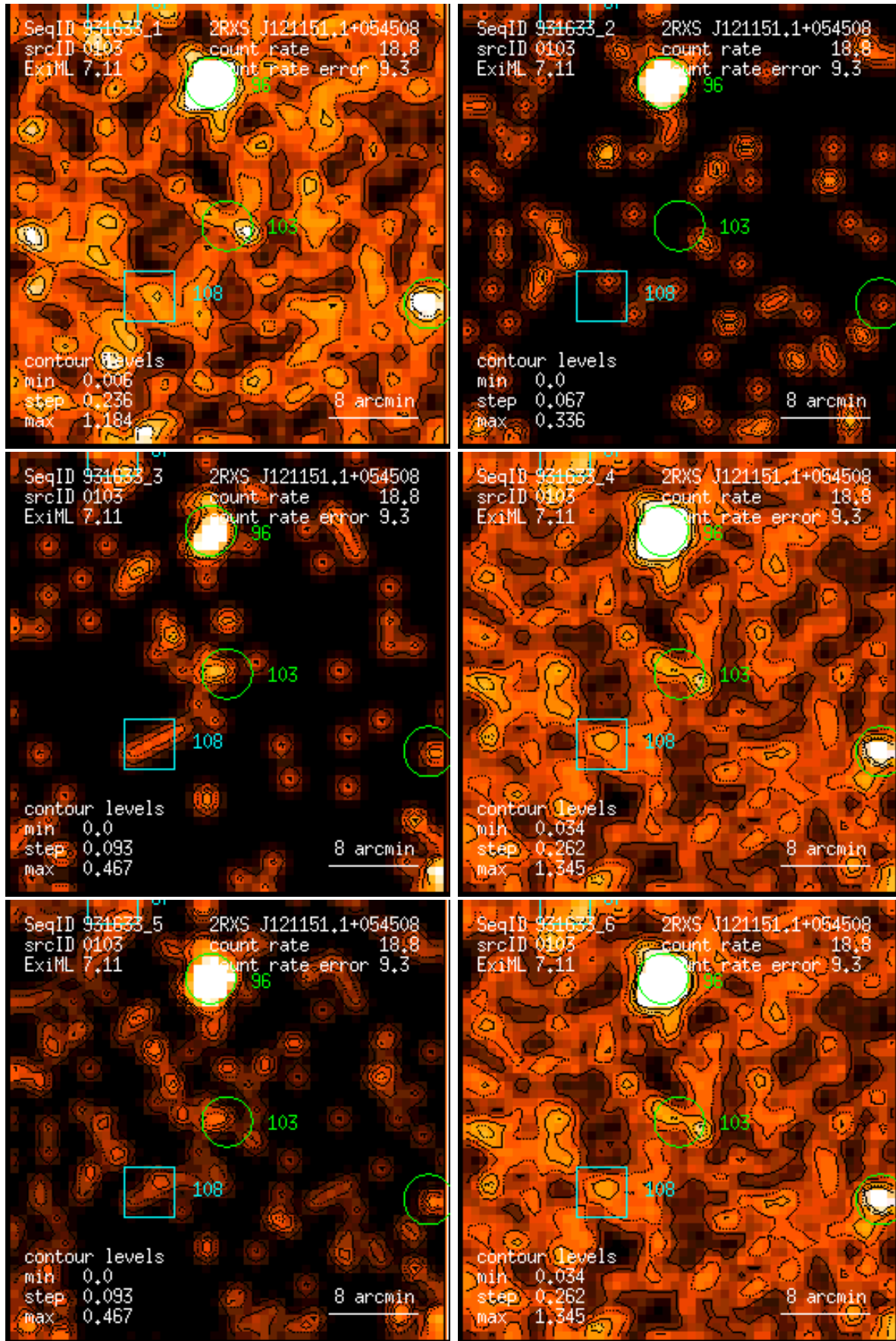
Figure 103: RASS 931633: detection 0103: band rate images, Gaussian filter: (1) PSPC channels 11 – 41, (2) 52 – 90, (3) 91 – 201, (4) 11 – 235, (5) 52 – 201, (6) 11 – 201. Broad band rates in counts/ks. Band rate contour levels in counts/ks/arcmin 2 .
