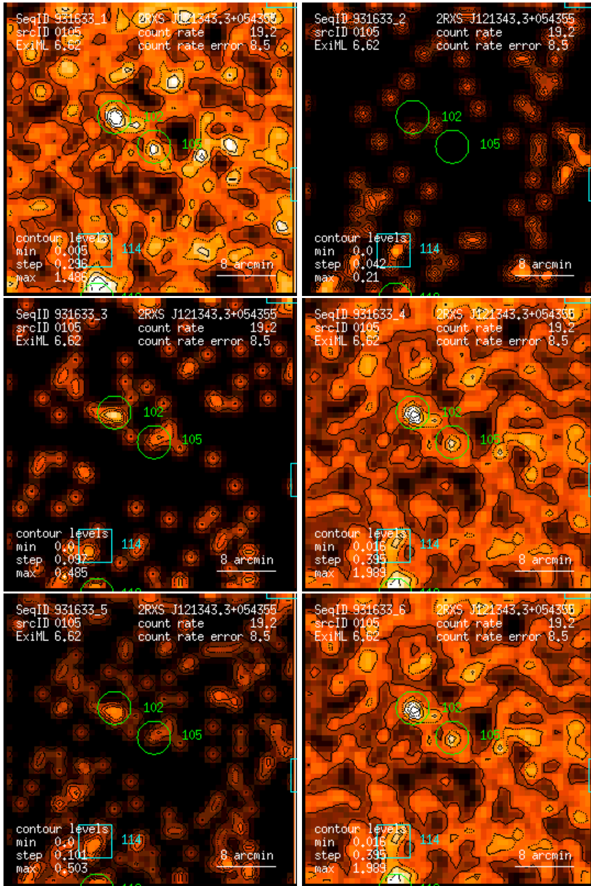
Figure 105: RASS 931633: detection 0105: band rate images, Gaussian filter: (1) PSPC channels 11 – 41, (2) 52 – 90, (3) 91 – 201, (4) 11 – 235, (5) 52 – 201, (6) 11 – 201. Broad band rates in counts/ks. Band rate contour levels in counts/ks/arcmin 2 .
