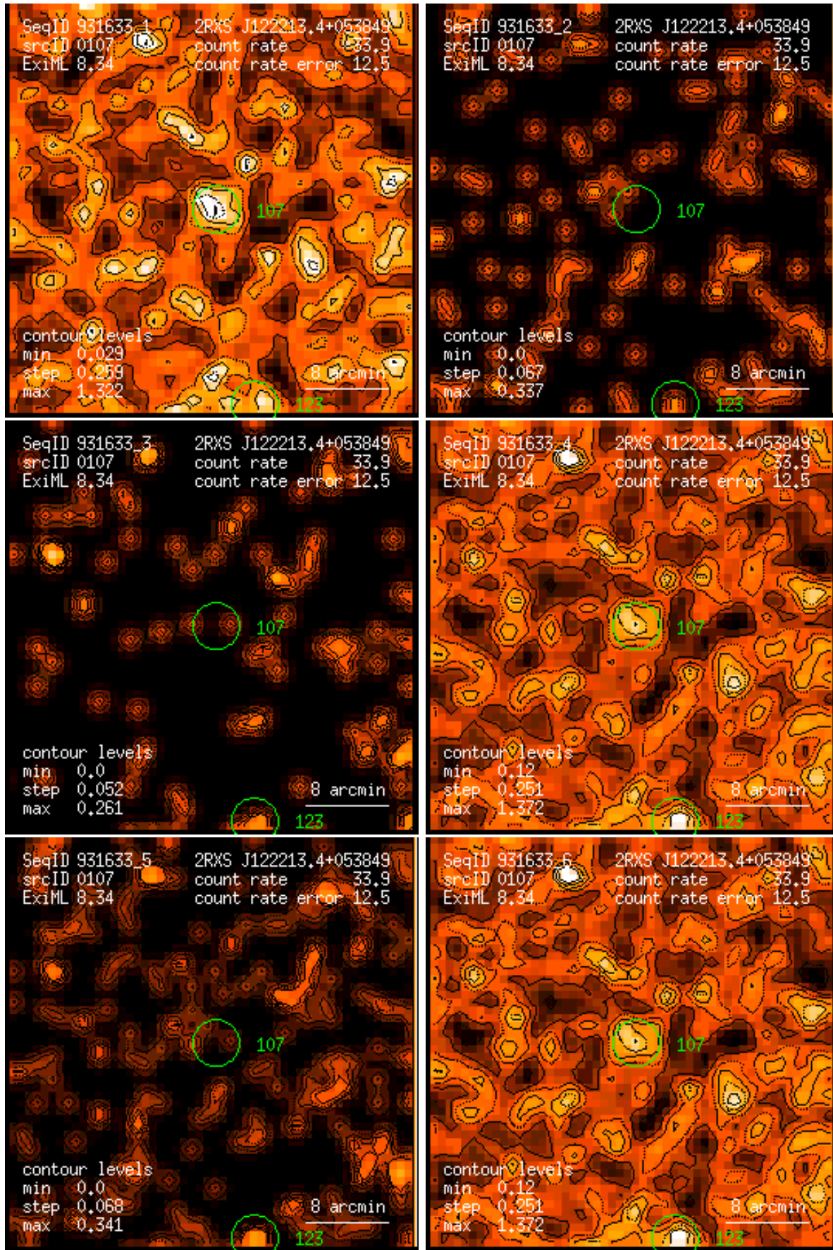
Figure 107: RASS 931633: detection 0107: band rate images, Gaussian filter: (1) PSPC channels 11 – 41, (2) 52 – 90, (3) 91 – 201, (4) 11 – 235, (5) 52 – 201, (6) 11 – 201. Broad band rates in counts/ks. Band rate contour levels in counts/ks/arcmin 2 .
