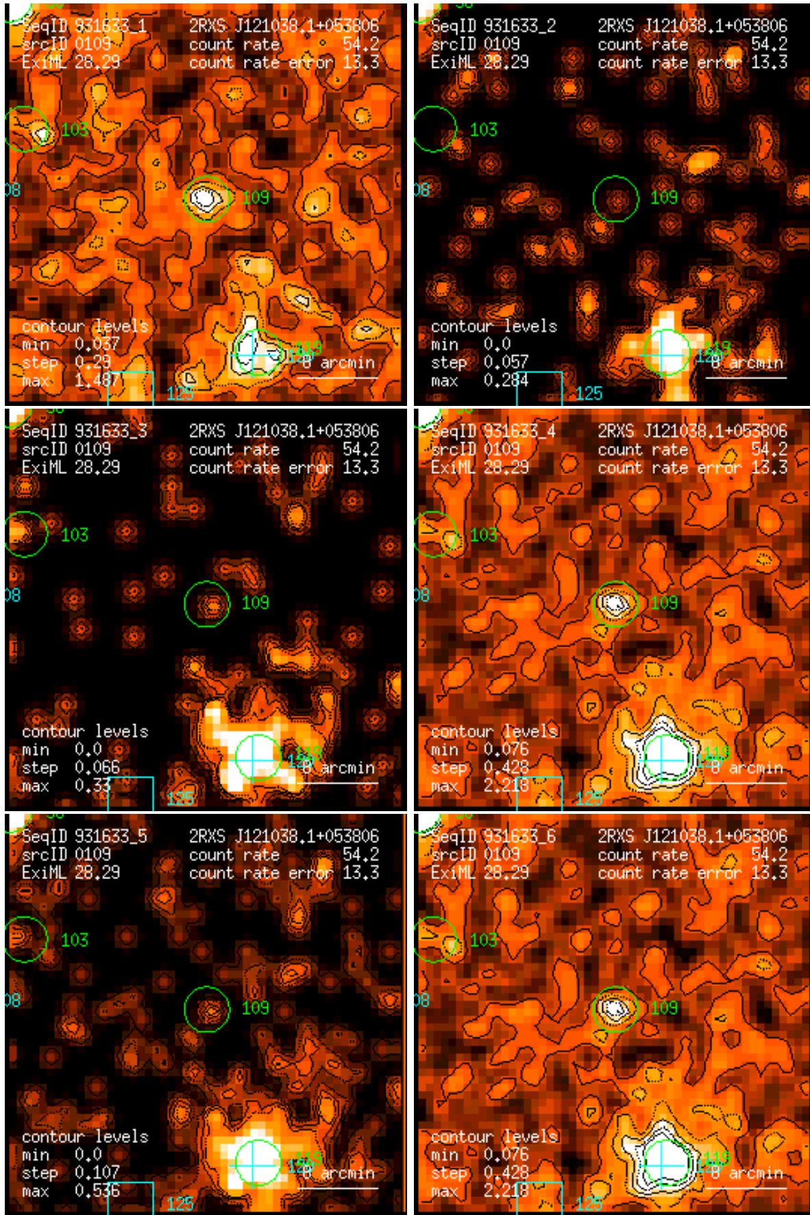
Figure 109: RASS 931633: detection 0109: band rate images, Gaussian filter: (1) PSPC channels 11 – 41, (2) 52 – 90, (3) 91 – 201, (4) 11 – 235, (5) 52 – 201, (6) 11 – 201. Broad band rates in counts/ks. Band rate contour levels in counts/ks/arcmin 2 .
