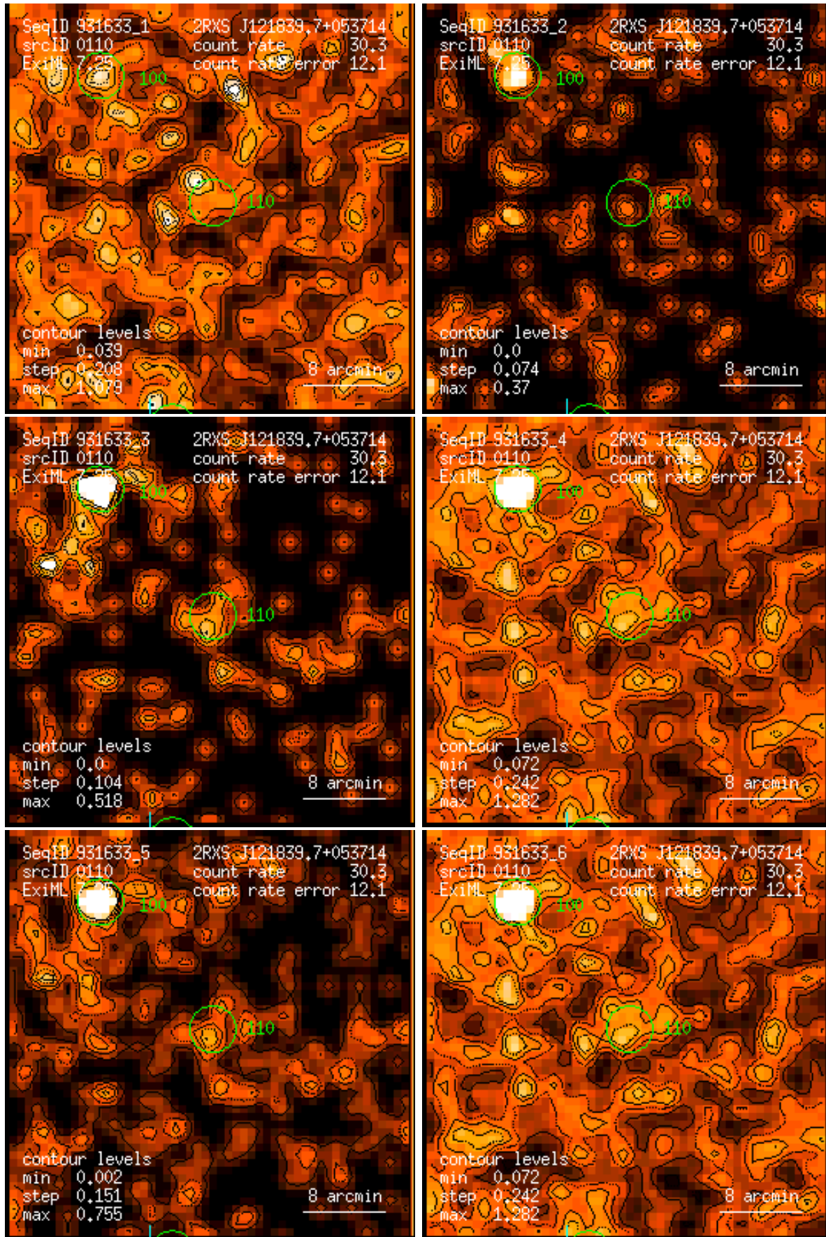
Figure 110: RASS 931633: detection 0110: band rate images, Gaussian filter: (1) PSPC channels 11 – 41, (2) 52 – 90, (3) 91 – 201, (4) 11 – 235, (5) 52 – 201, (6) 11 – 201. Broad band rates in counts/ks. Band rate contour levels in counts/ks/arcmin 2 .
