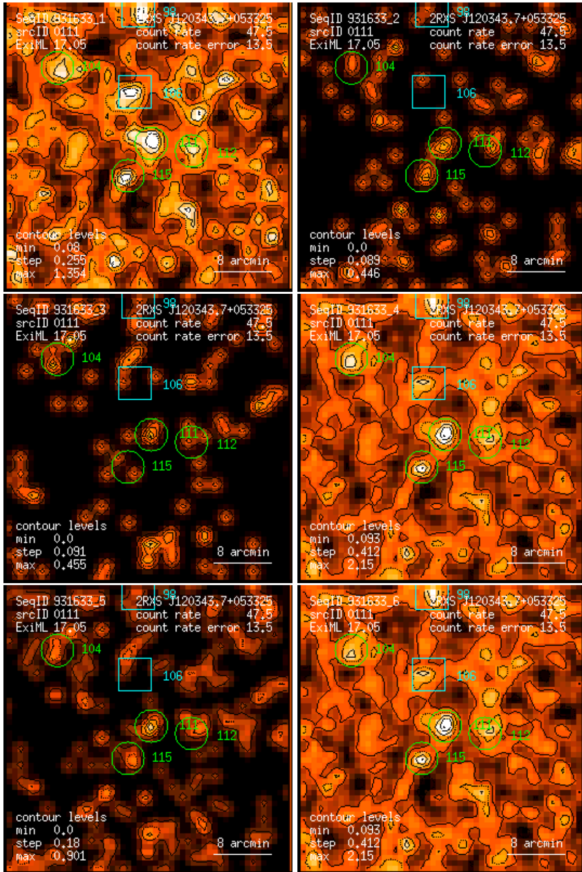
Figure 111: RASS 931633: detection 0111: band rate images, Gaussian filter: (1) PSPC channels 11 – 41, (2) 52 – 90, (3) 91 – 201, (4) 11 – 235, (5) 52 – 201, (6) 11 – 201. Broad band rates in counts/ks. Band rate contour levels in counts/ks/arcmin 2 .
