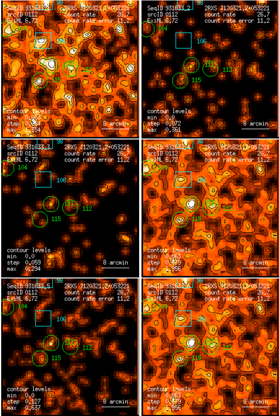
Figure 112: RASS 931633: detection 0112: band rate images, Gaussian filter: (1) PSPC channels 11 – 41, (2) 52 – 90, (3) 91 – 201, (4) 11 – 235, (5) 52 – 201, (6) 11 – 201. Broad band rates in counts/ks. Band rate contour levels in counts/ks/arcmin 2 .
